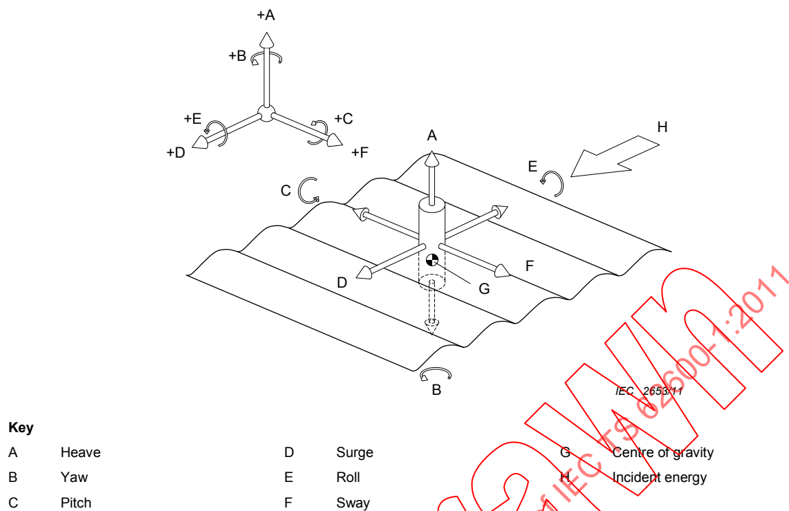
Figure 1 – Six degrees of freedom – Floating device
