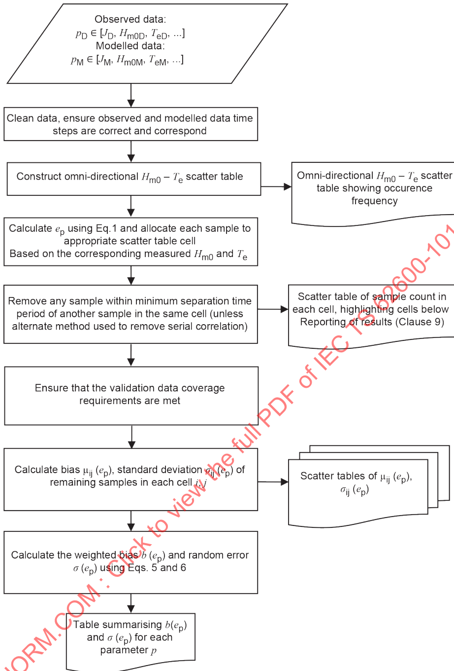
Figure 2 – Validation flow chart
