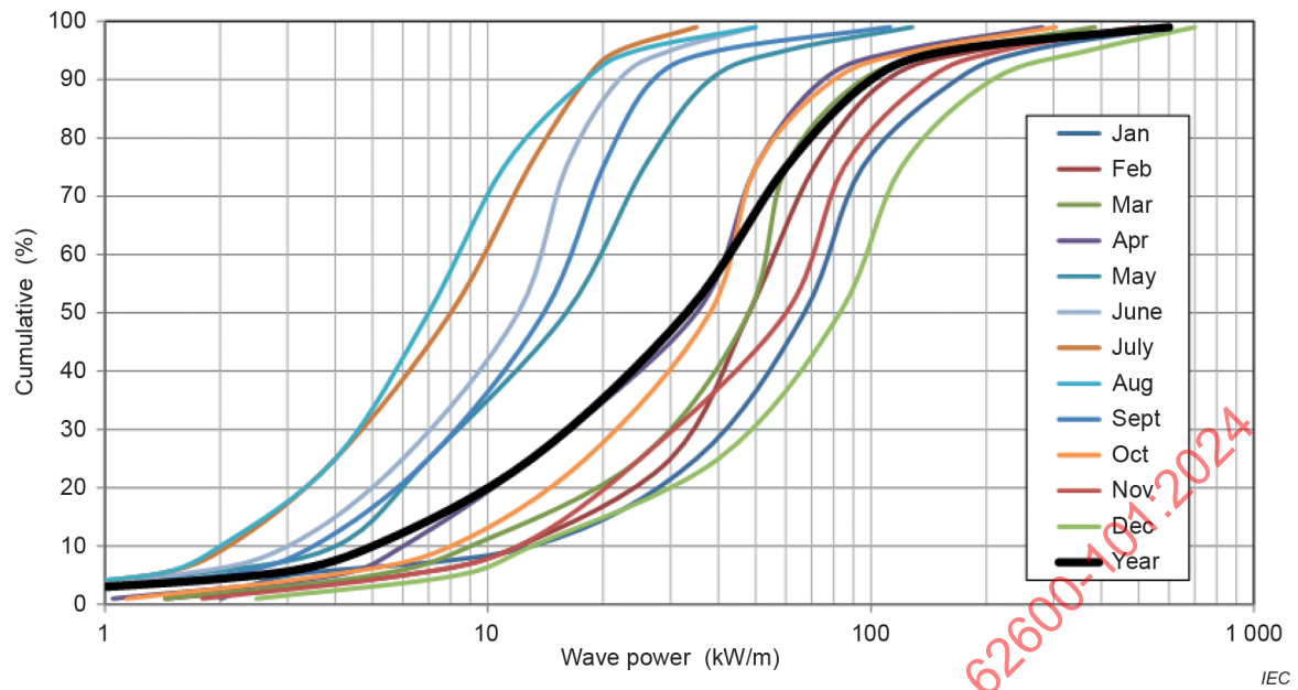
Figure 6 – Example plot showing the distribution of wave power for different months
