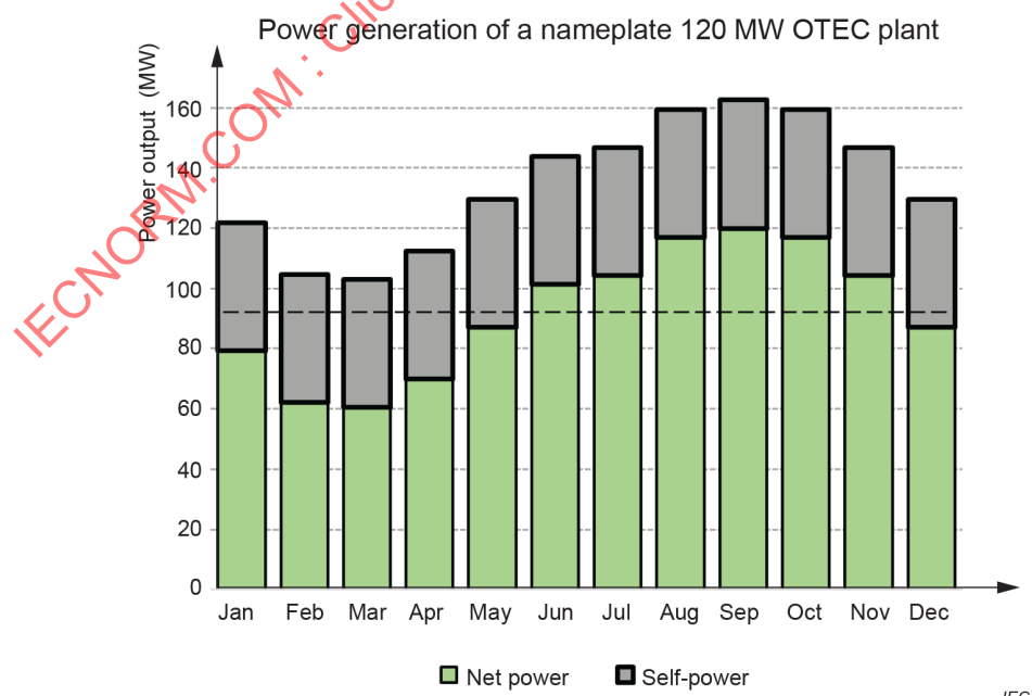
Figure 7 – Example of OTEC power definitions
