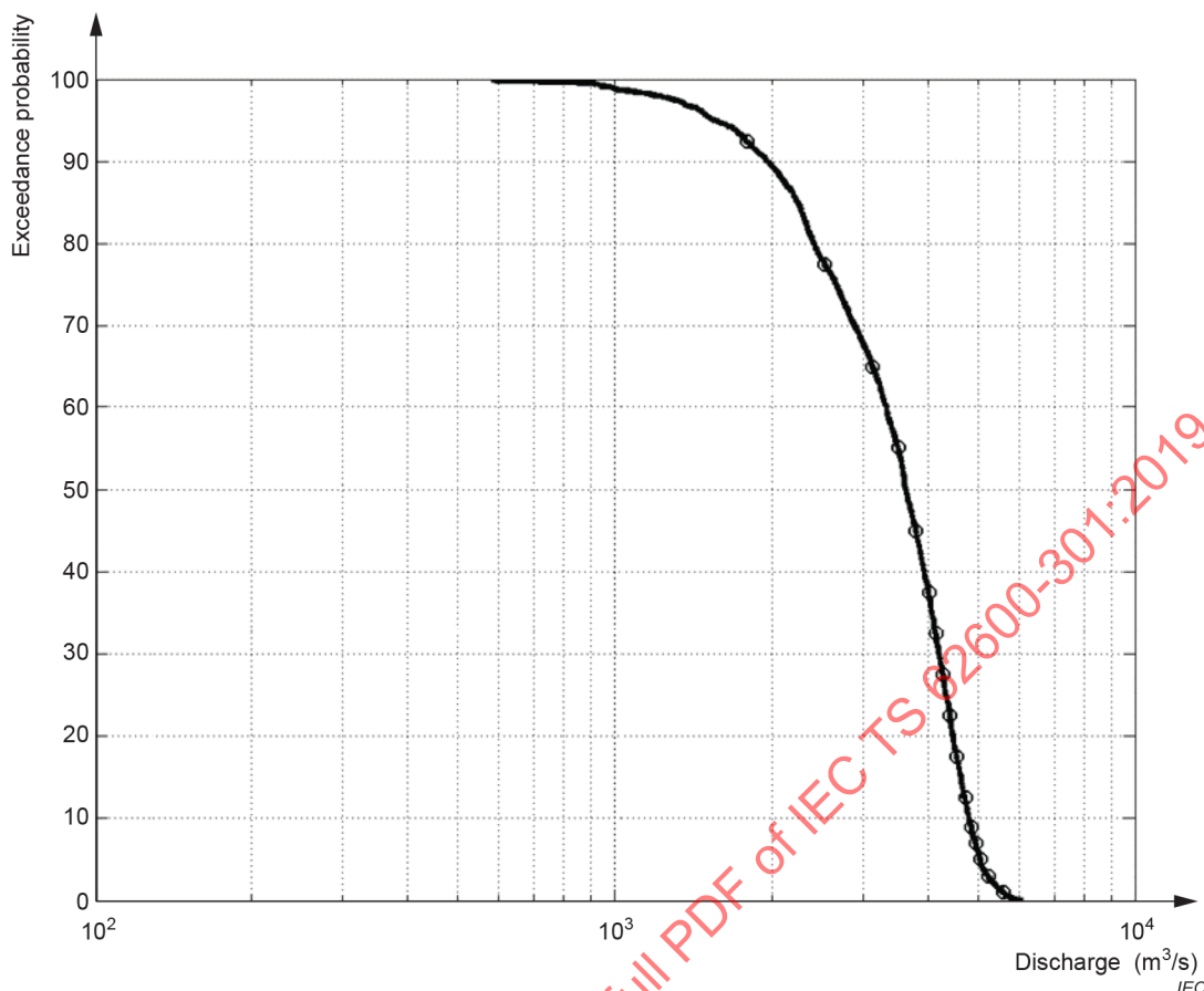
Figure 3 – Example FDC (curve) and assumed non-uniform discretisation (circles)
