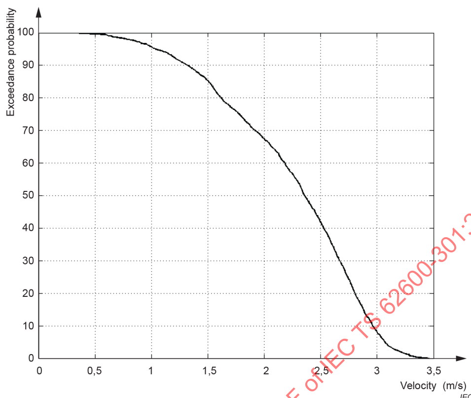
Figure 5 – Example VDC using the transfer function derived from the curve fit shown in Figure 4 and the full FDC shown in Figure 3
