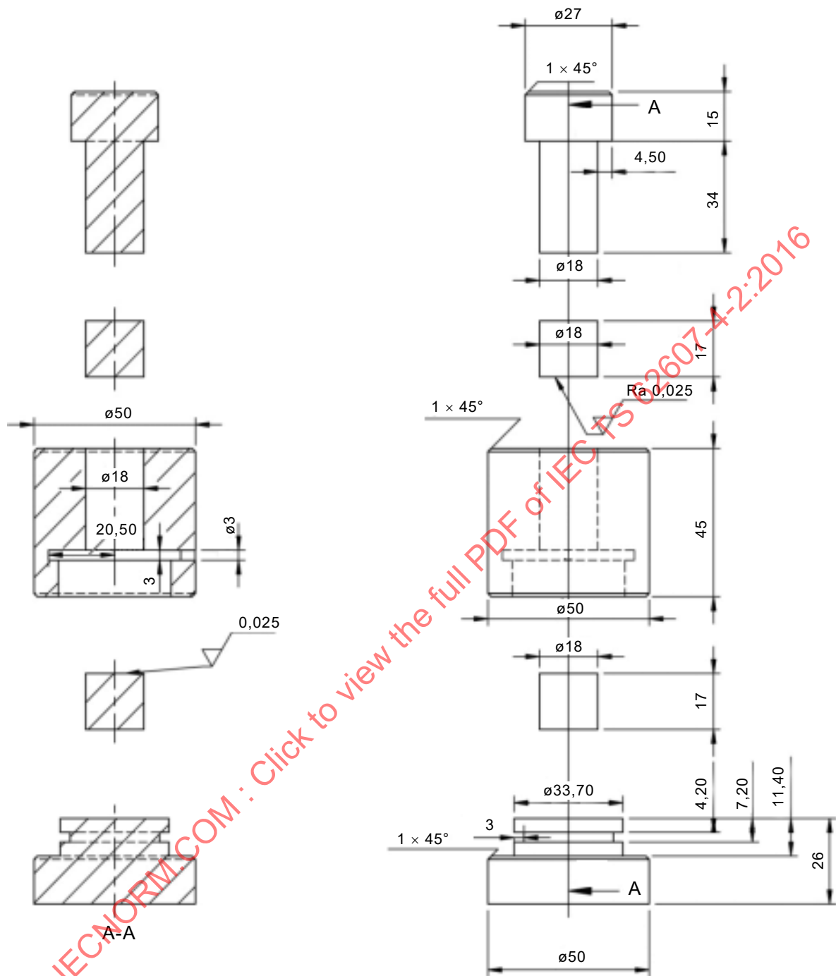
Figure A.2 – Engineering schematic of die for compacted density measurement
