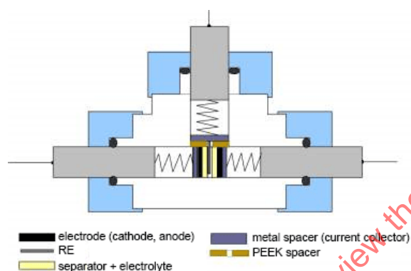
Figure A.1 – 3-electrode screw cell
