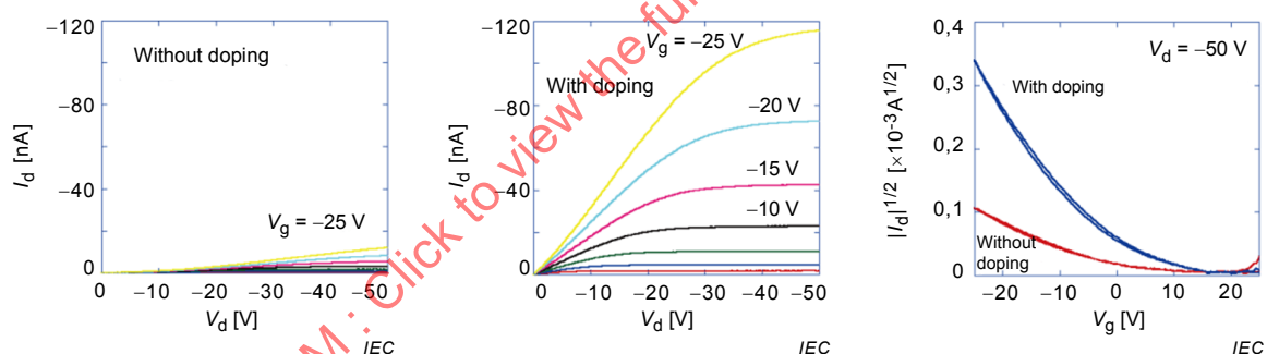
a) Drain current-drain voltage curves for oligothiophene BGBC OTFT without carrier-doped layers
