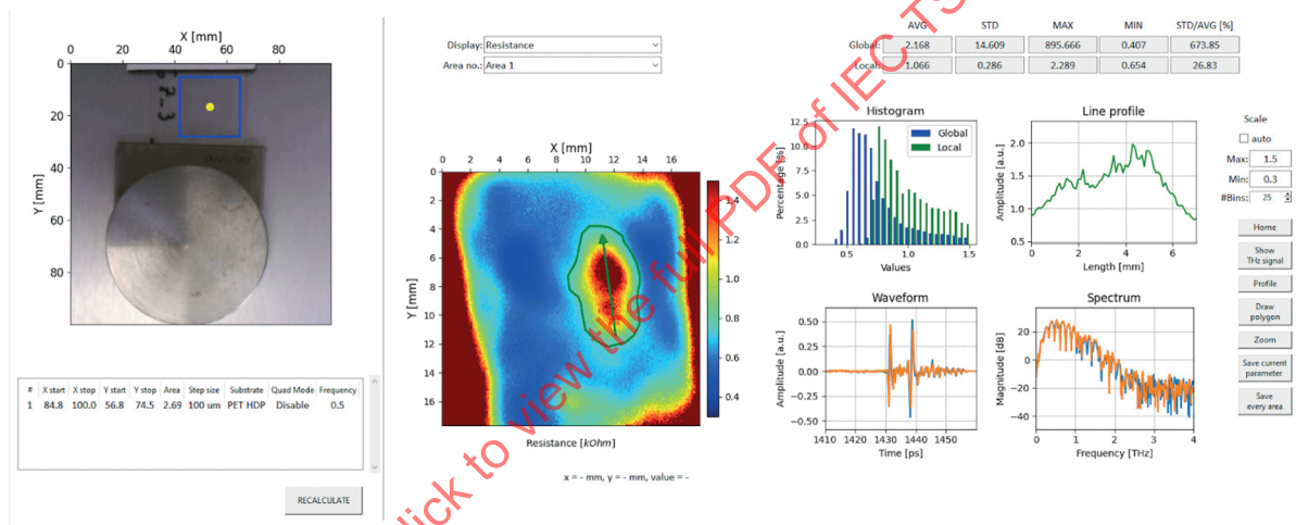
Figure 10 – Analysis of low-resistance areas in the resistance map
