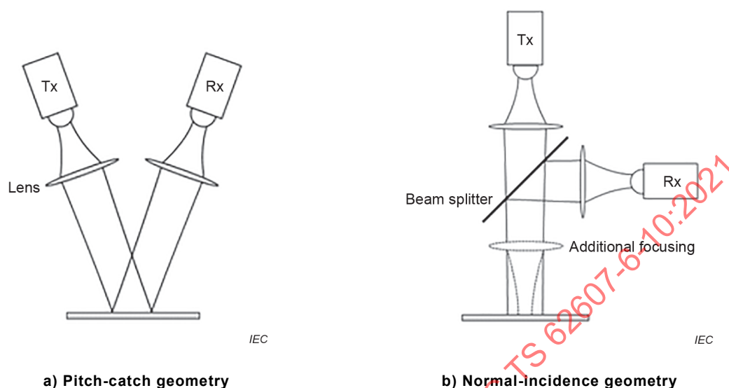
Figure 5 – Comparison of different reflection geometries
