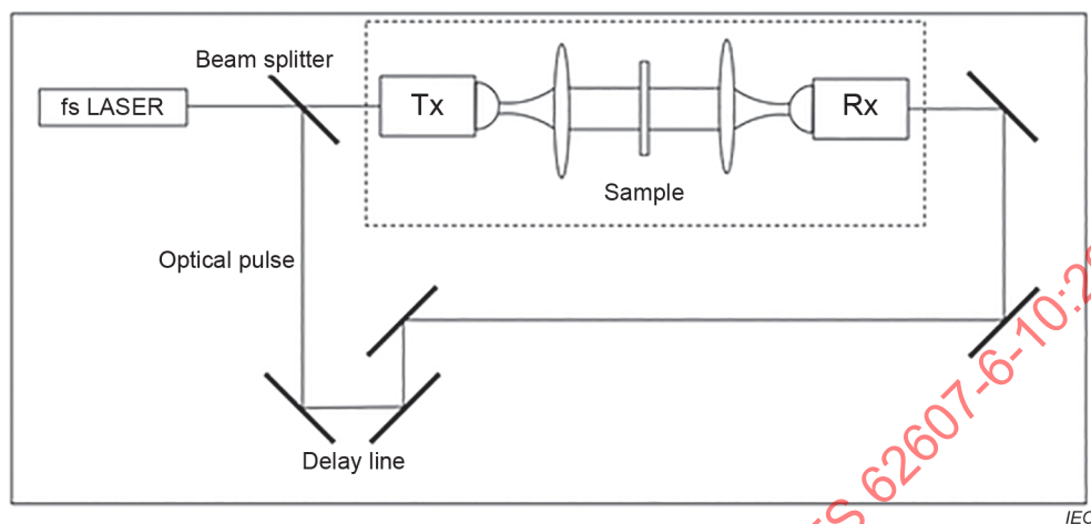
Figure 3 – Principal components of a classical THz-TDS system
