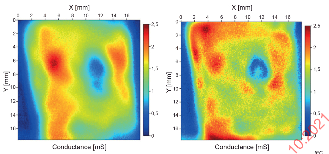
Figure 12 – Conductance maps at two different frequencies: 0,5 THz and 0,75 THz
