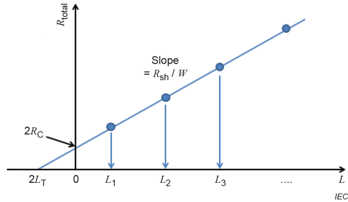
Figure 2 – Determination of contact resistance and sheet resistance
