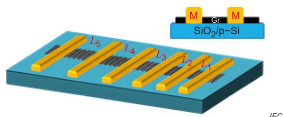
a) schematic views of the graphene TLM pattern
