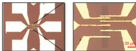
b) optical microscopy images of the TLM pattern
