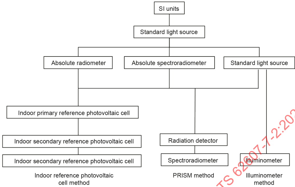
Figure 2 – Calibration chain example
