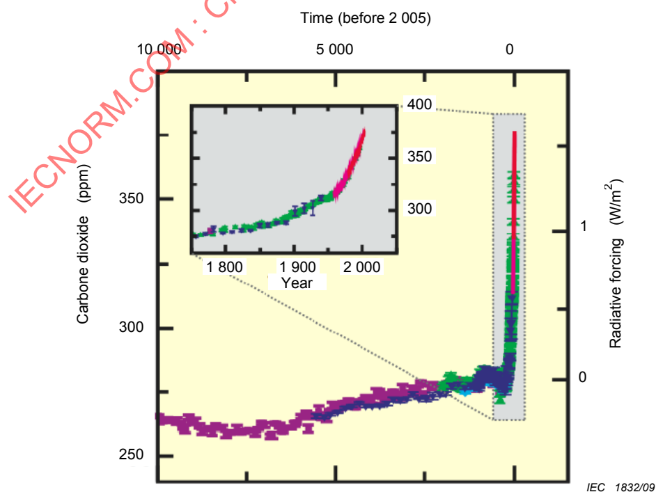
Figure A.2 – Changes in greenhouse gases from ice-core and modern data [5]
