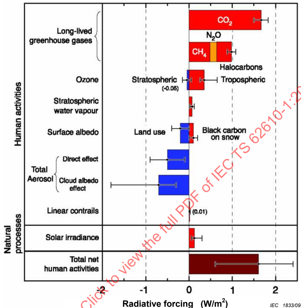
Figure A.3 – Radiative forcing of climate between 1750 and 2005 [4]
