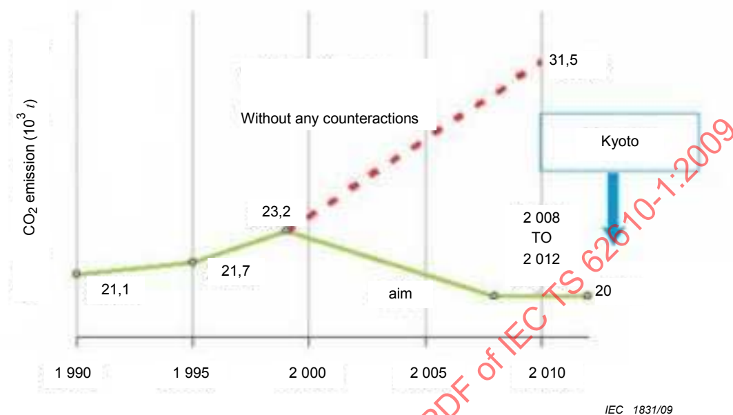
Figure A.1 – Current CO 2 emission situation
