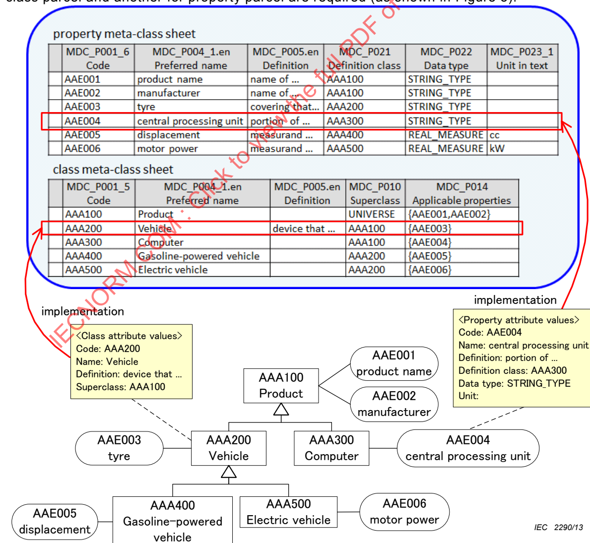
Figure 3 – Spreadsheet implementation
