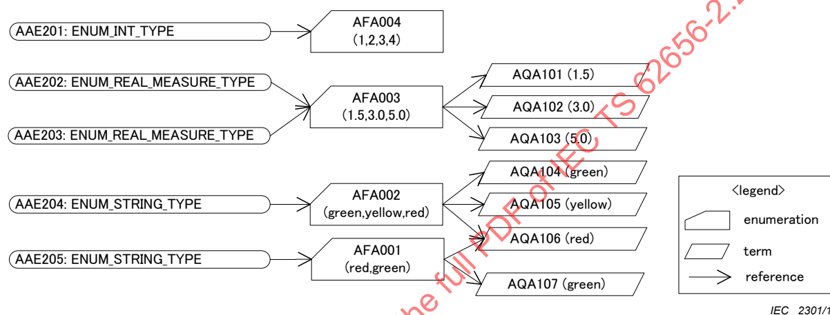
Figure 14 – Example of a use case of enumeration
