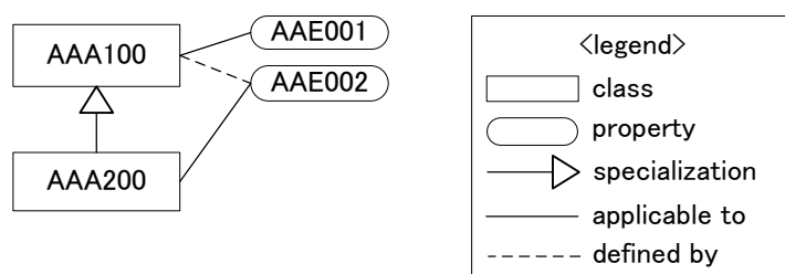
Figure 7 – Example of a simple classification tree
