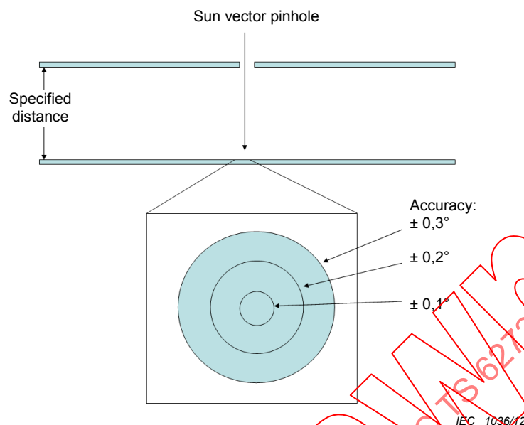
Figure 4 – Two flat parallel plates at a specified distance, one having a pin hole for sunlight to be tracked on specified-diameter circles that ultimately measure 0,1°, 0,2°, and 0,3° accuracy rings (more if necessary)
