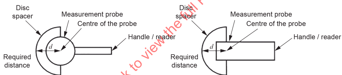
Figure A.1 – Disc spacer around two types of measurement probes
