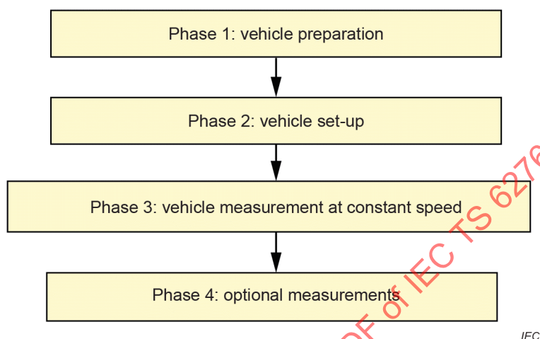
Figure 3 – Specific driving mode set-up and test
