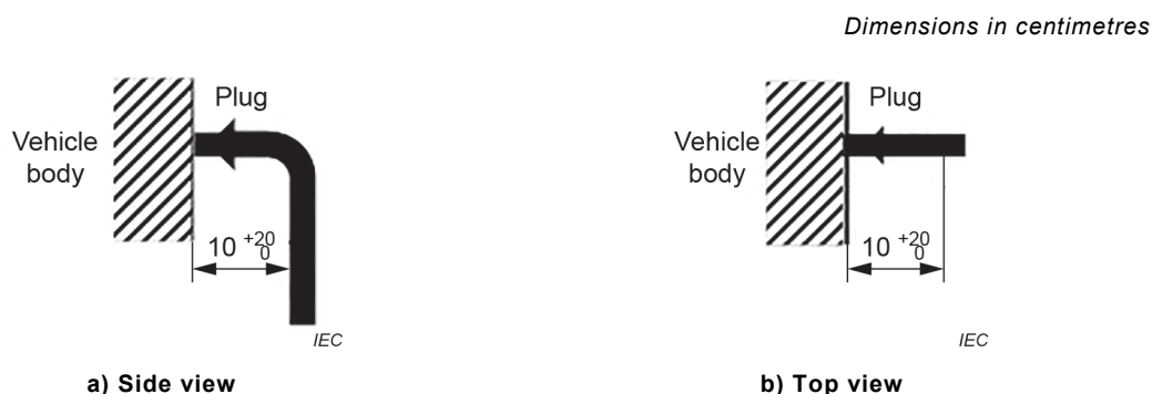
Figure 6 – Plug-in charging supply cable positioning
