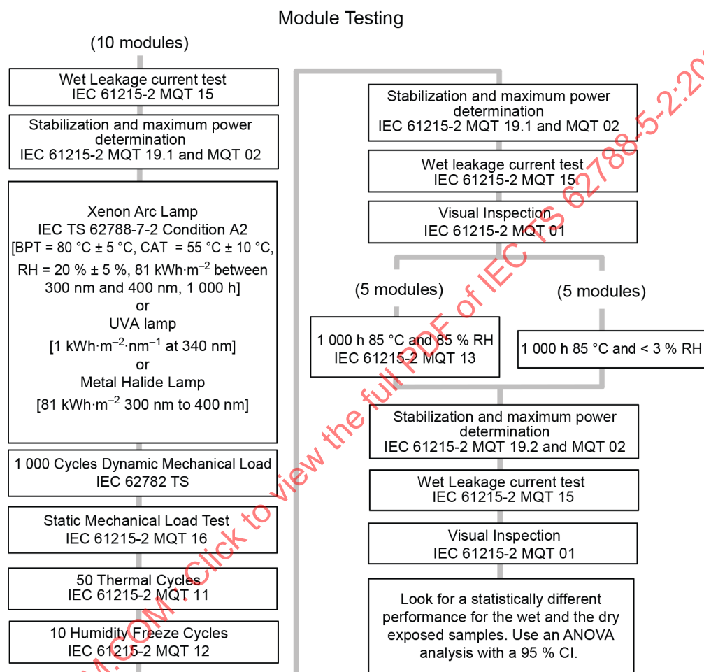
Figure 3 – Module test flow diagram
