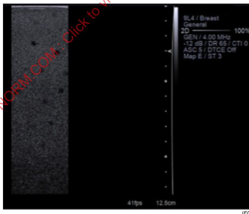
Figure B.5 – One of 80 parallel linear-array images of the phantom containing 4 mm-diameter, low-echo spheres, at 4 MHz with focus at 3 cm
