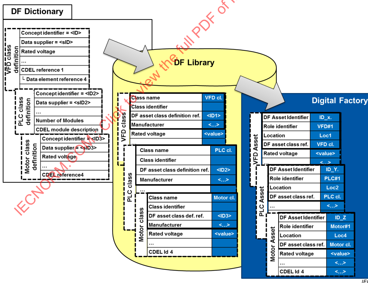
Figure 9 – Example of DF asset and DF asset class
