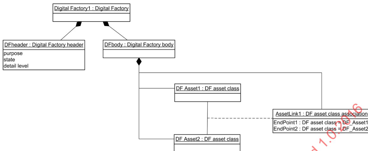
Figure A.8 – Digital Factory
