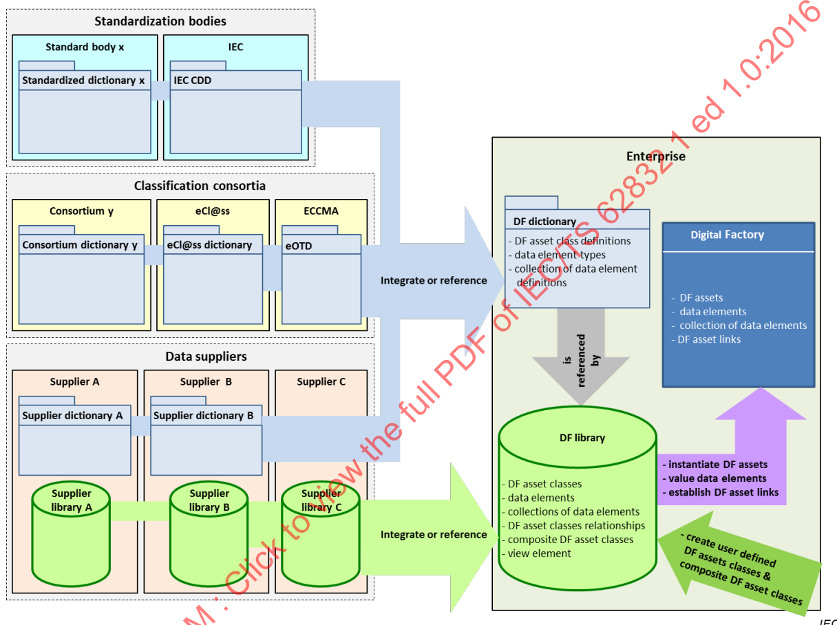
Figure 1 – DF framework overview
