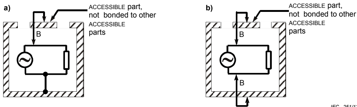
Figures D.2 a) and b) – Protection between a HAZARDOUS LIVE internal circuit and an ACCESSIBLE part which is not bonded to other ACCESSIBLE parts
