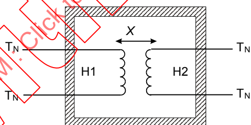
Figures D.2 c) and d) – Protection between a HAZARDOUS LIVE primary circuit and circuits which have ACCESSIBLE external TERMINALS
