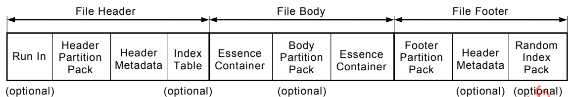
Figure 1 – Overview of MXF file structure
