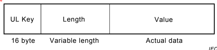
Figure 3 – Key-length-value encoding
