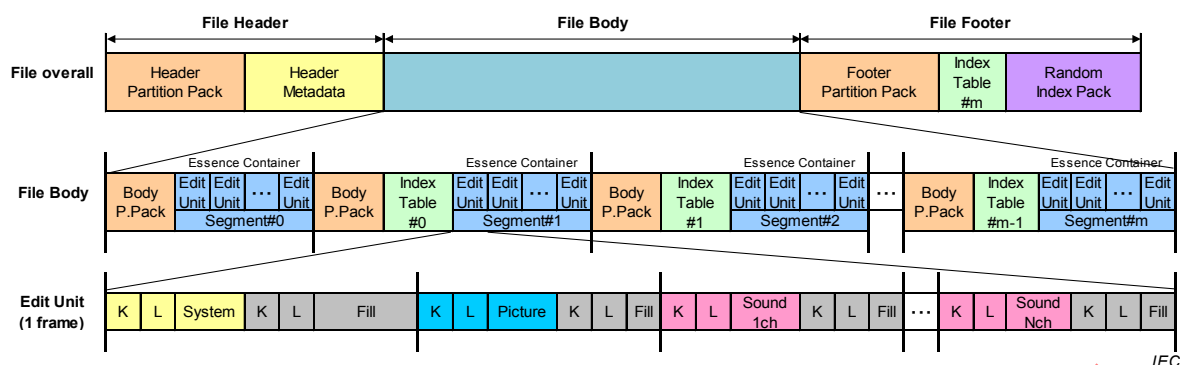
Figure 7 – Typical example of Index Table placement for OP-1a
