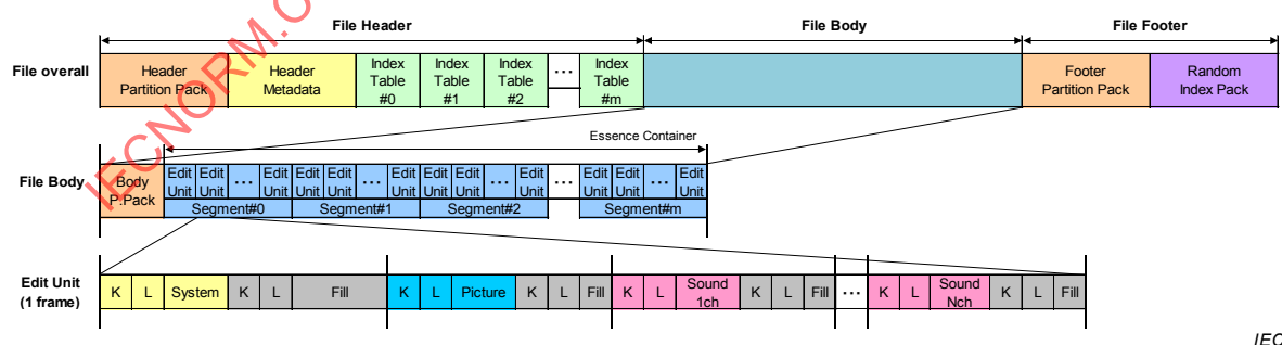
Figure 9 – Example-2 to locate the entire Index Table in the Header Partition
