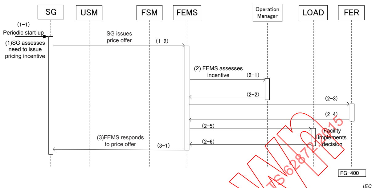
Figure A.5 – Sequence diagram for FG-400
