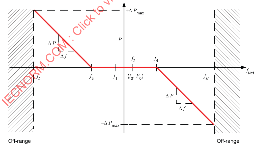
Figure 3 – The P-f control in isolated microgrid
