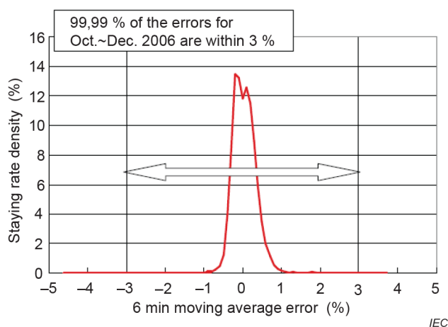
Figure A.17 – Performances for grid connected operation: deviation from planned flow
