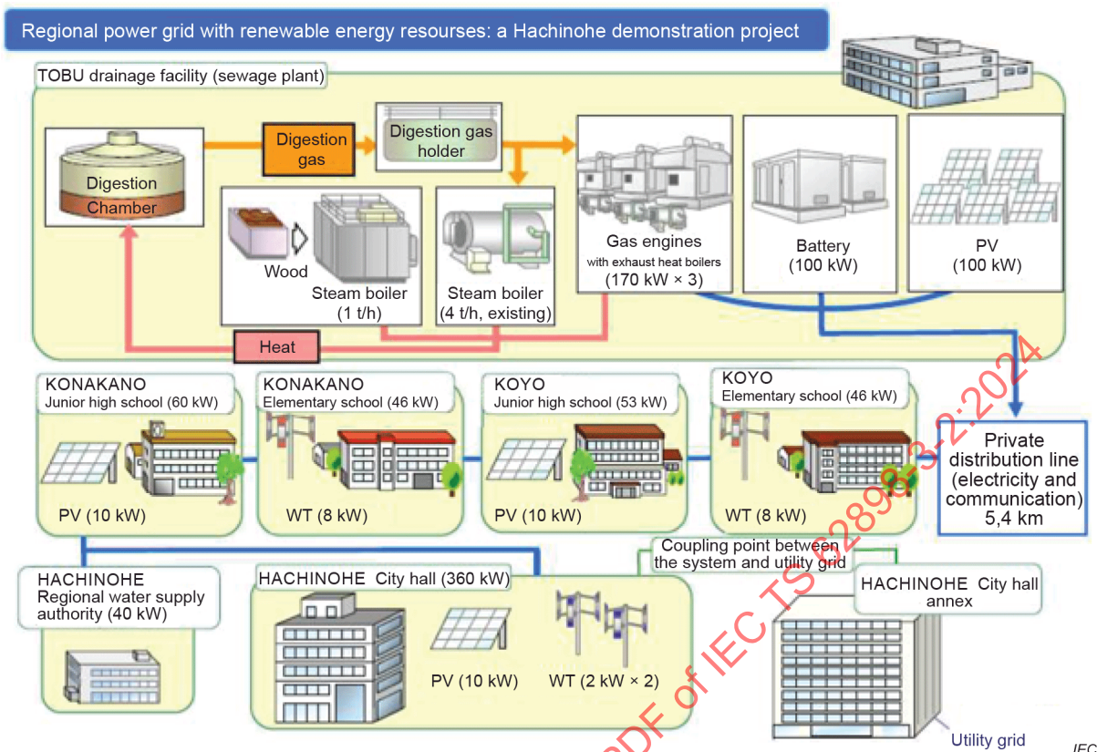
Figure A.15 – Overview of Hachinohe demonstration project
