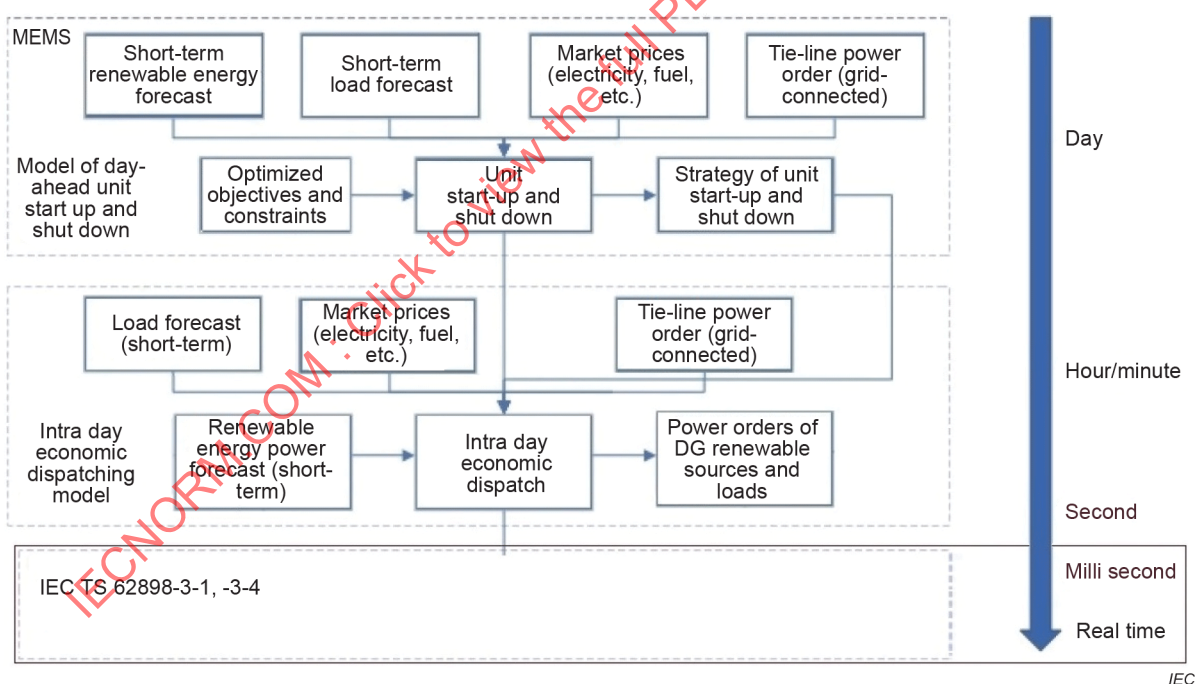
Figure 5 – Microgrid energy management system functional architecture
