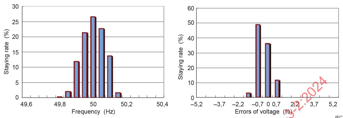
Figure A.18 – Obtained success rate of maintaining frequency and voltage
