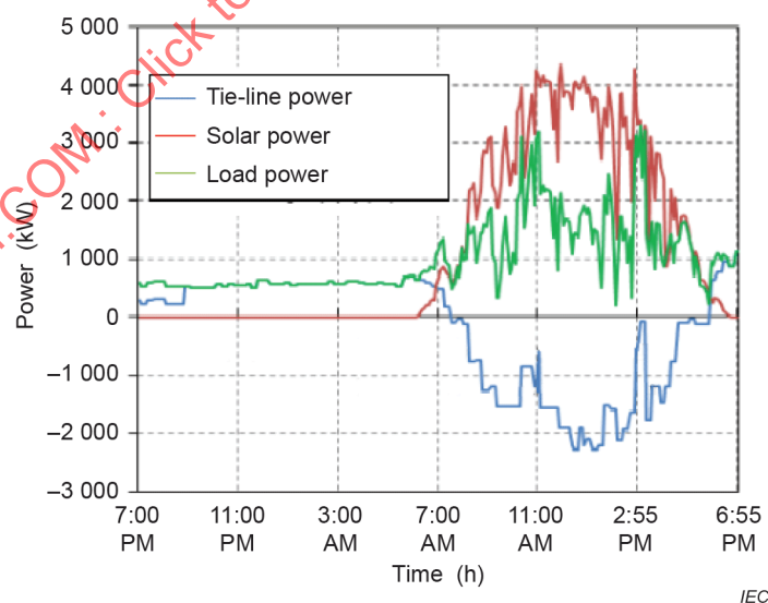
Figure A.13 – Example of power generation and consumption detailed on a particular day in Foshan industrial microgrid
