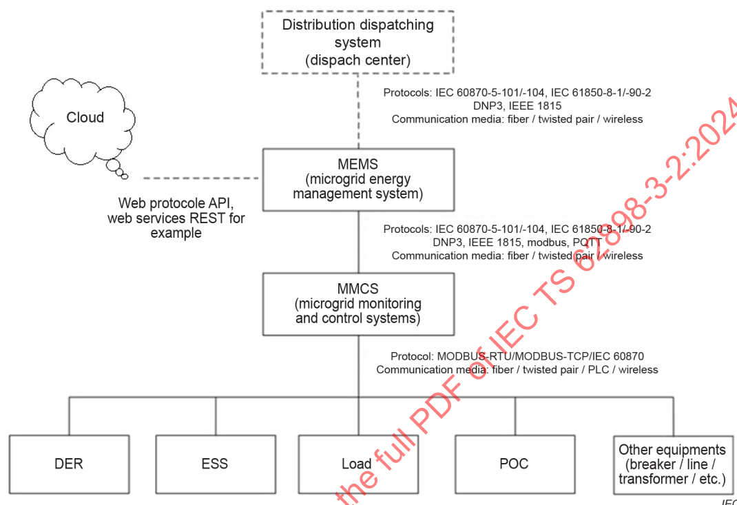
Figure 3 – Typical three-layer communication for structure 1
