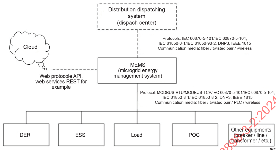
Figure 4 – Typical two-layer communication for structure 2
