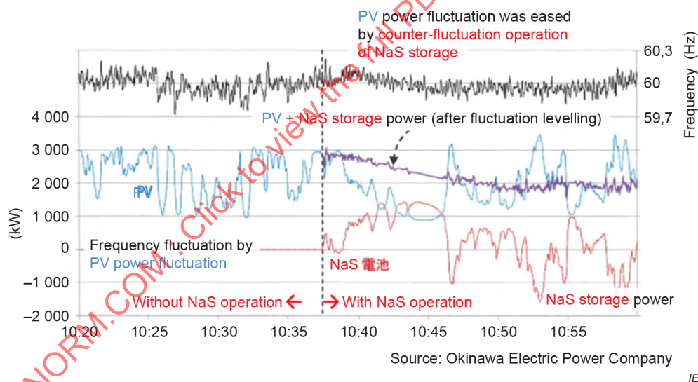
Figure A.28 – Result of the PV + NaS storage long term operation
