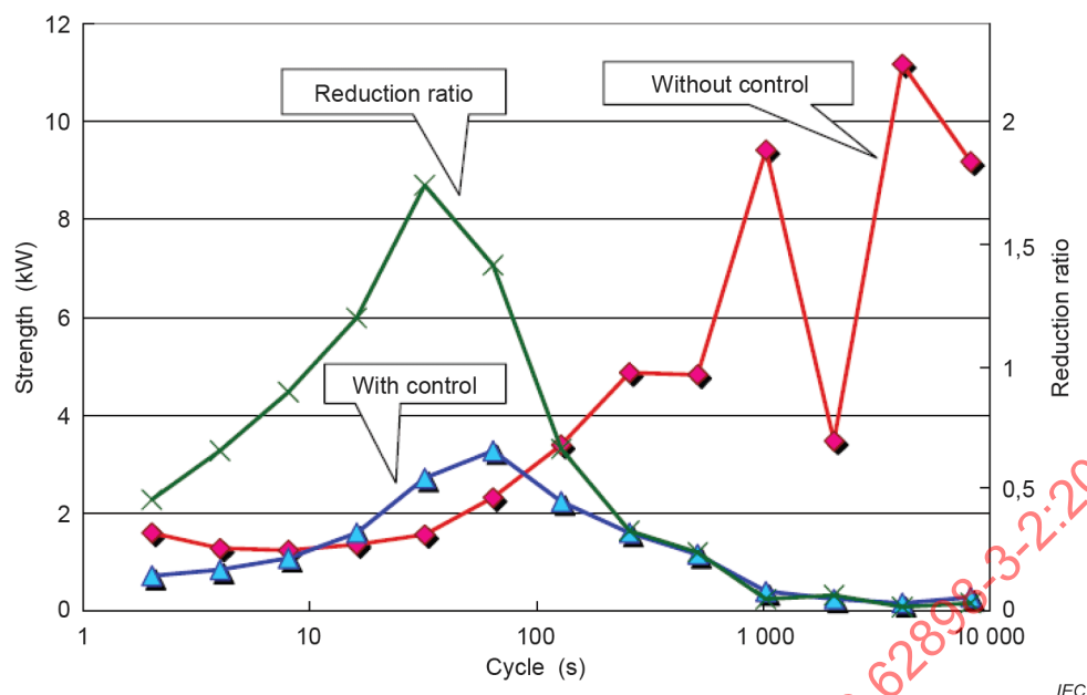
Figure A.19 – Overall performance under different battery operation modes
