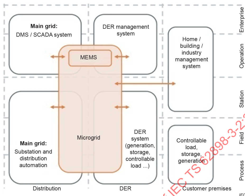
Figure 1 – Conceptual map of a power system consisting of a microgrid
