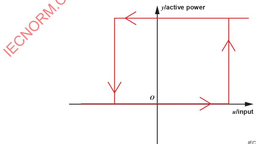
Figure 1 – Hysteresis curve of a switchable load
