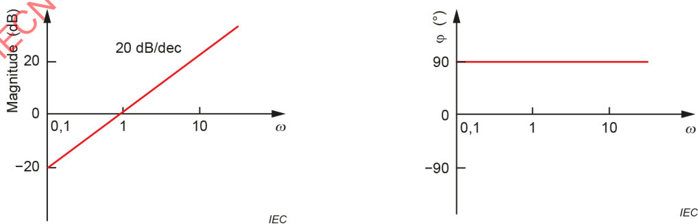
Figure 4 – Bode diagram of a typical differential loop
