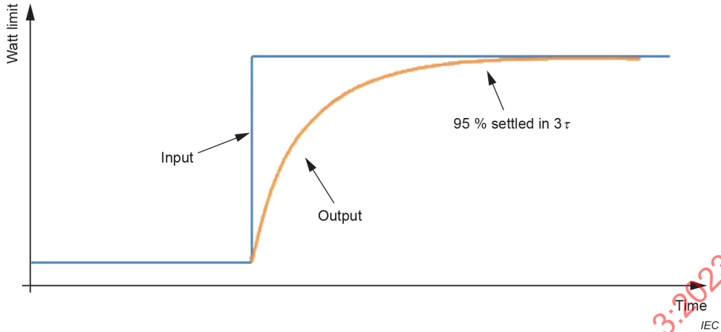
Figure 5 – Time domain response of first order low-pass filter
