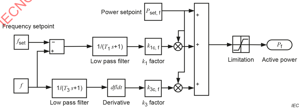
Figure 6 – Functional diagram of a combined frequency control function for continuously controllable dispatchable loads
