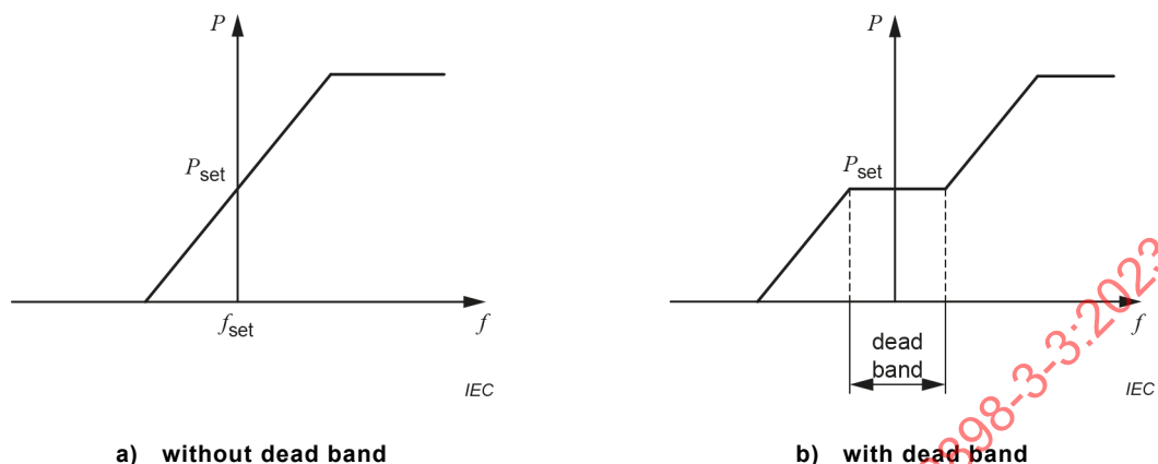
Figure 3 – Example of P(f) self-regulation before and after activating the dead band
