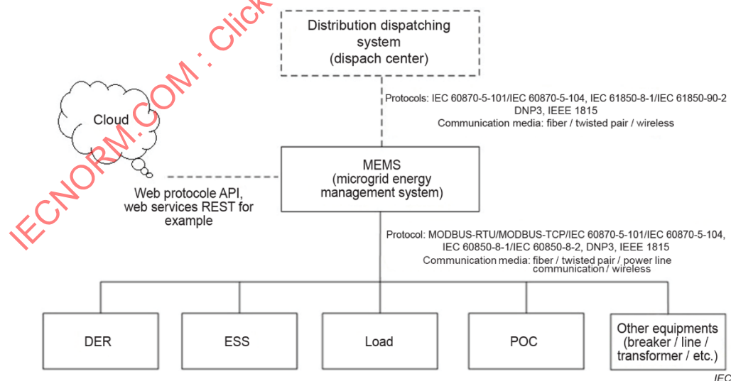
Figure 4 – Typical two-layer communication for structure 2
