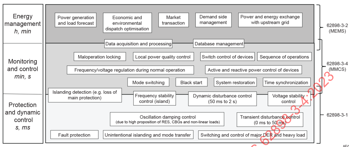
Figure 1 – Functional mapping for operation and control of microgrids
