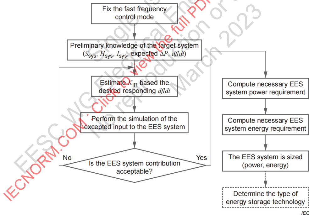
Figure 20 – Example of EES system sizing process for fast frequency control
