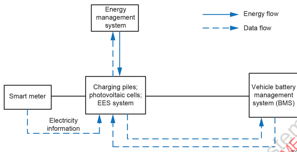
Figure 41 – Example of electric charging stations monitoring system architecture in combination with renewable energy sources and EES system
