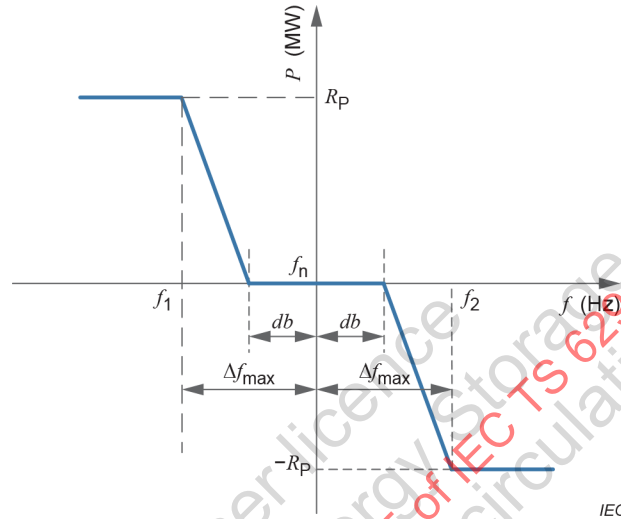
Figure 8 – Example of droop control with frequency dead band
