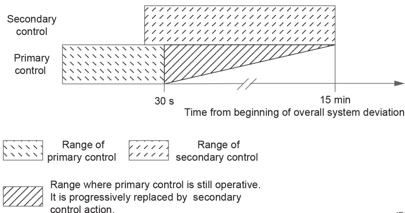
Figure 6 – Example of frequency regulation time/duration schematic diagram
