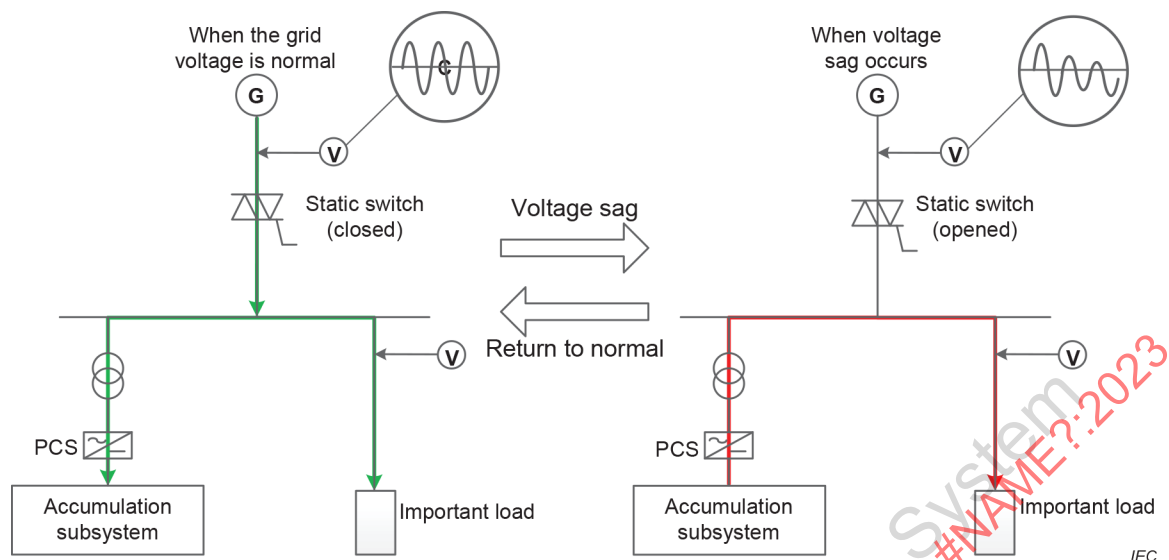
Figure 29 – Example of control strategy for the voltage sag mitigation application
