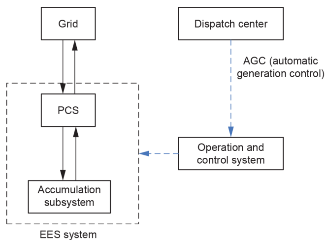
Figure 13 – Example of EES system participating in secondary frequency regulation
