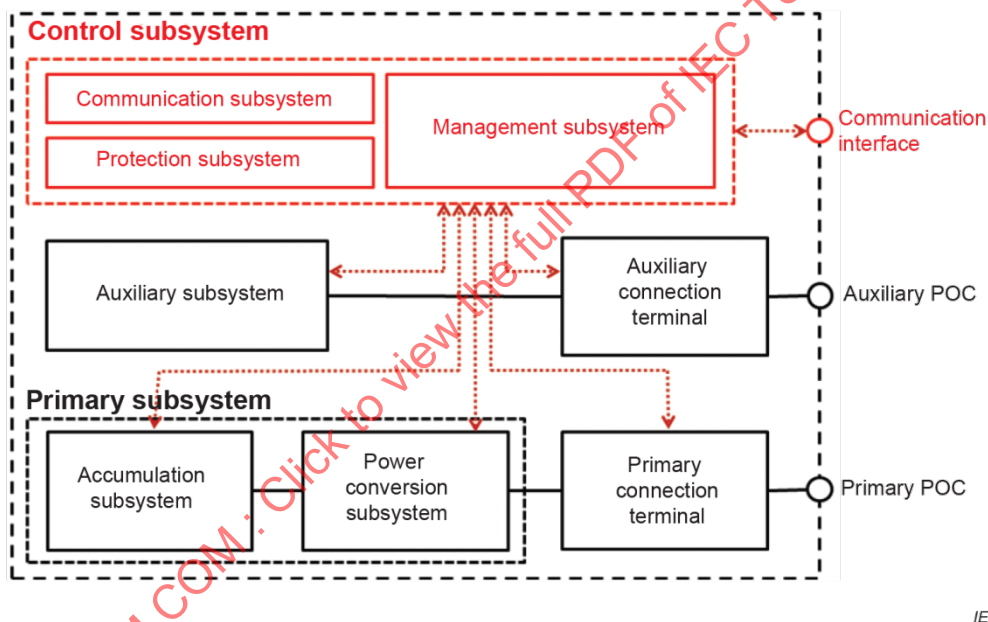
b) EES system with auxiliary POC
