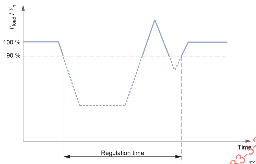
Figure 27 – Example of regulation time of the EES system for voltage sag mitigation
