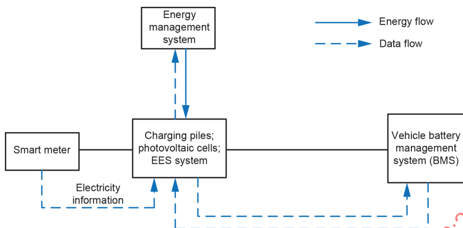
Figure 41 – Example of electric charging stations monitoring system architecture in combination with renewable energy sources and EES system
