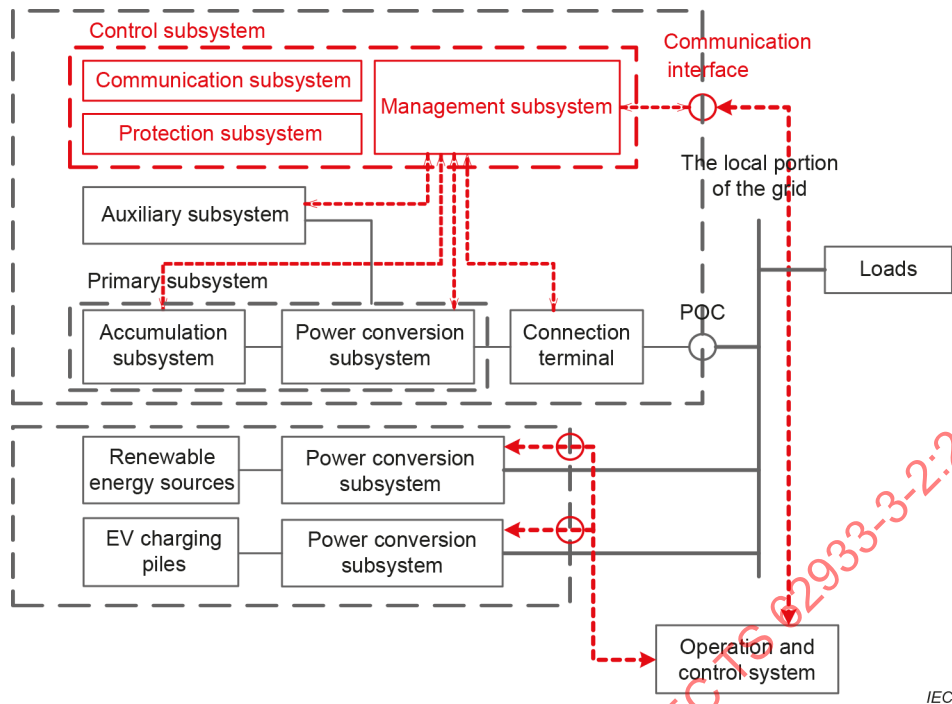
Figure 38 – Example of the system structure of the EES system in electric charging stations in combination with renewable energy sources
