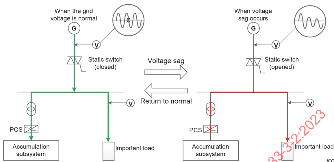
Figure 29 – Example of control strategy for the voltage sag mitigation application
