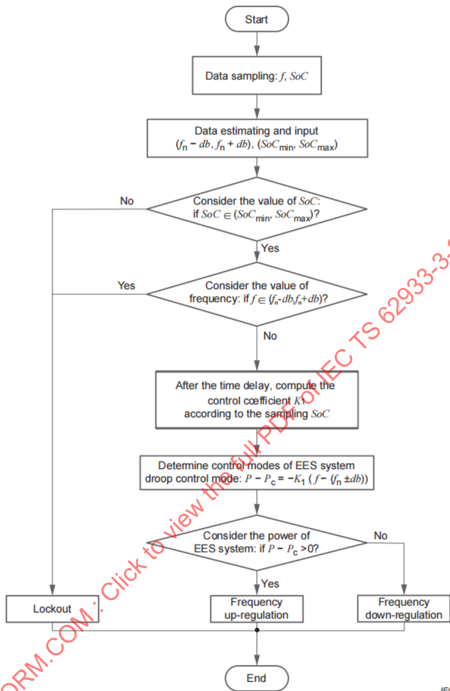
Figure 11 – Example of control strategy of the EES system participating in primary frequency regulation
