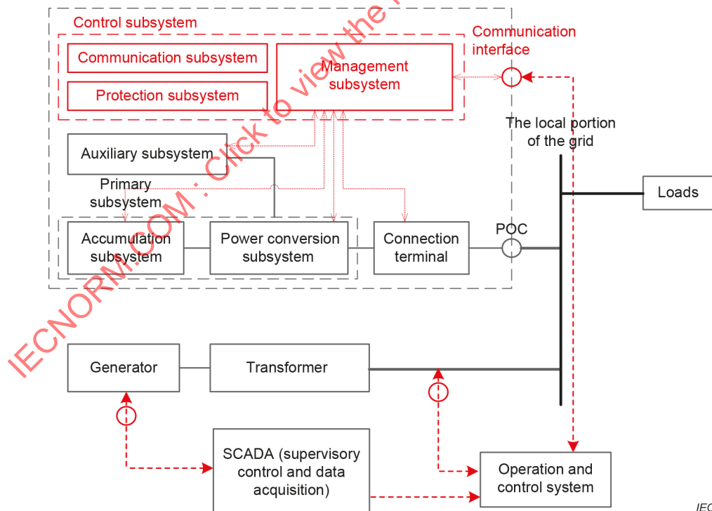
Figure 7 – Example of the system structure of the EES system for frequency regulation in conjunction with generator
