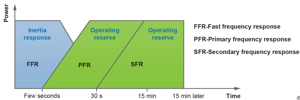
Figure 16 – Example of operation regions of different frequency response types
