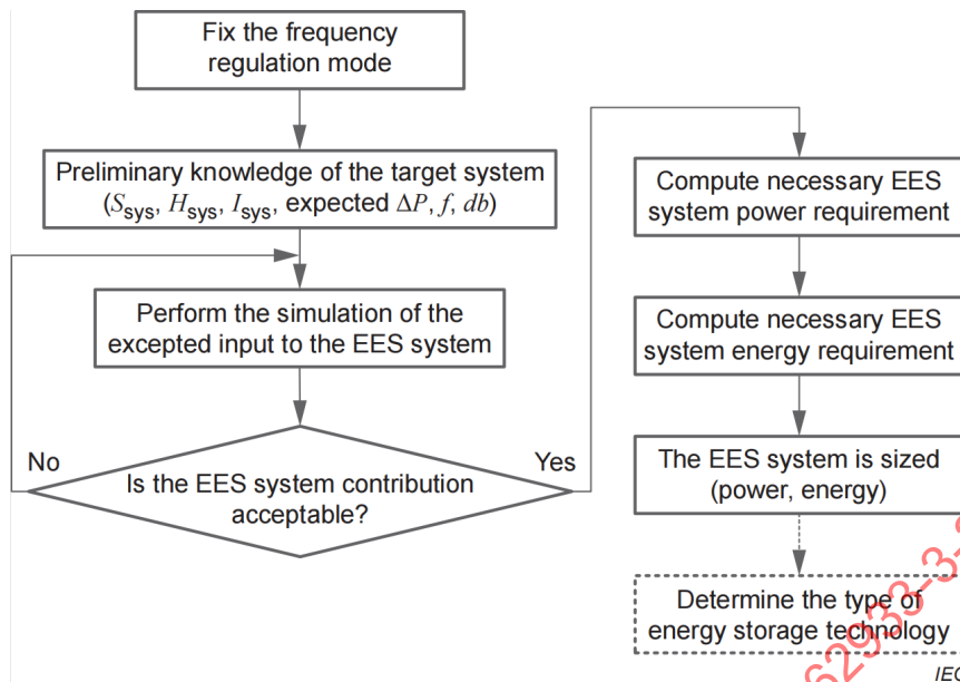
Figure 10 – Example of EES system sizing process for secondary frequency regulation
