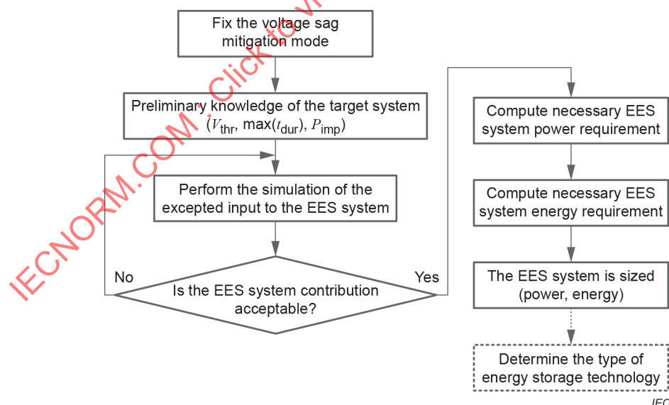
Figure 30 – Example of EES system sizing process for voltage sag mitigation
