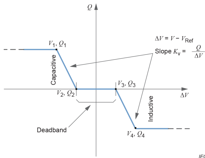
Figure 23 – Example of reactive voltage support schematic diagram
