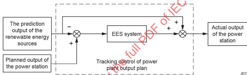
Figure 36 – Example of control strategy for the renewable energy sources (energy) firming application
