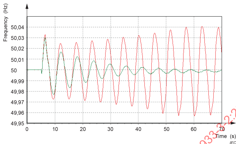
Figure 44 – Example of damping power oscillation simulation with five BESSs in a transmission grid
