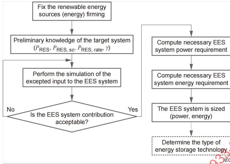
Figure 37 – Example of EES system sizing process for renewable energy sources (energy) generation firming
