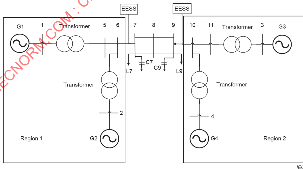
Figure 43 – Schematic diagram of typical four-generators two-regions system structure connected with the EES system
