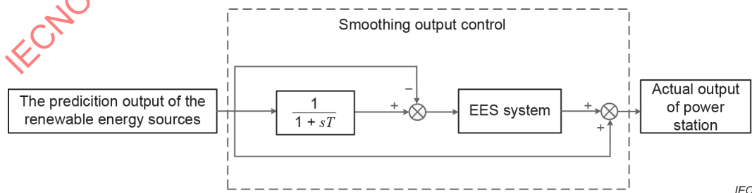
Figure 32 – Example of control strategy for the renewable energy sources (power) smoothing application
