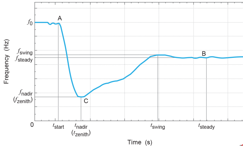
Figure 15 – Example of frequency curve with fast frequency control
