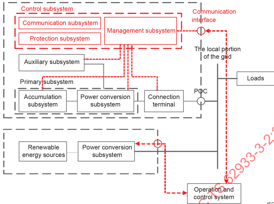
Figure 31 – Example of the system structure of the EES system connected with renewable energy sources
