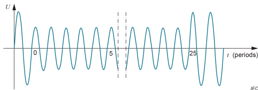
Figure 25 – Example of voltage sag
