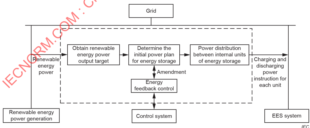
Figure 34 – Example of renewable energy sources (power) smoothing basic procedures
