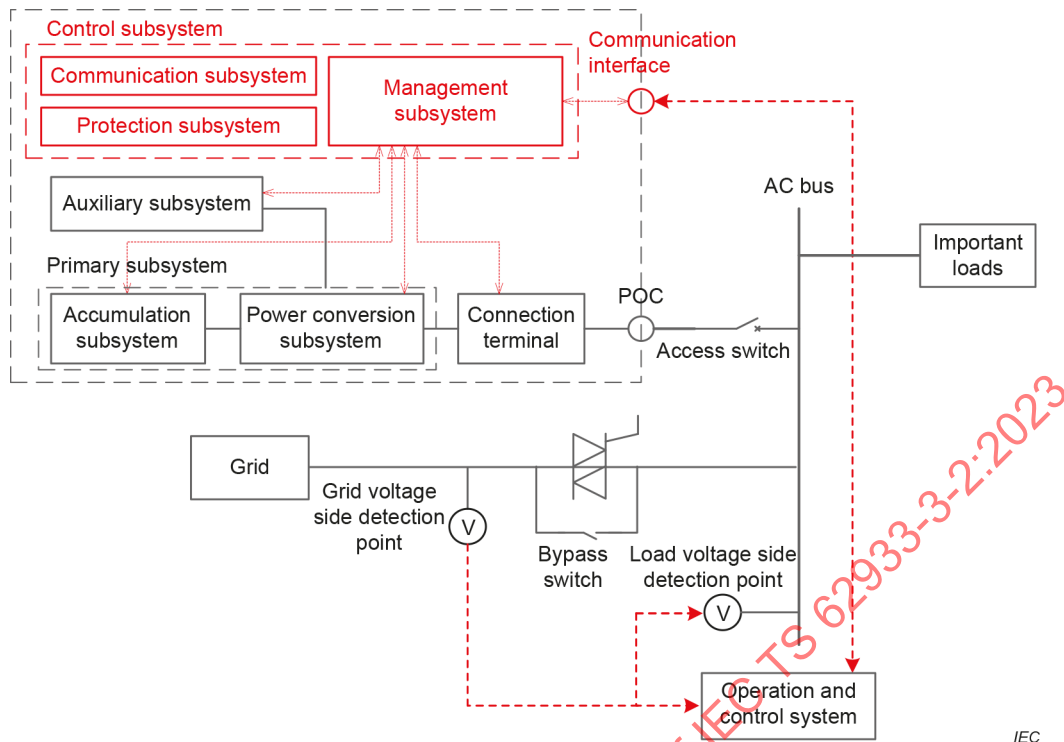
Figure 28 – Example of the system structure of the EES system for voltage sag mitigation
