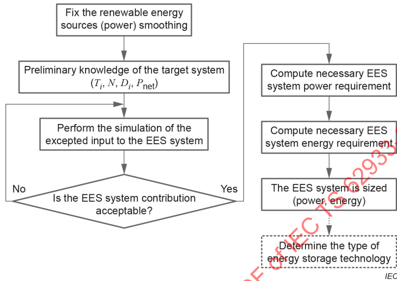
Figure 33 – Example of the EES system sizing process for renewable energy sources (power) smoothing
