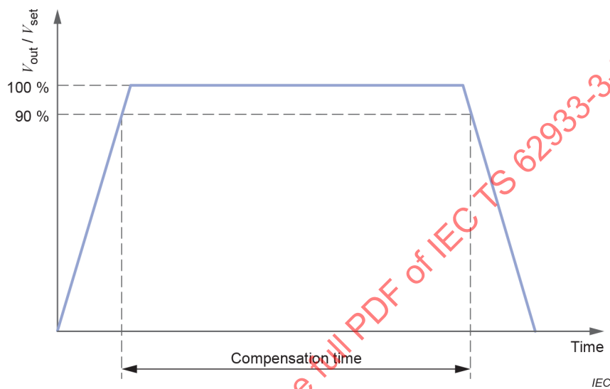
Figure 26 – Example of compensation time of the EES system for voltage sag mitigation
