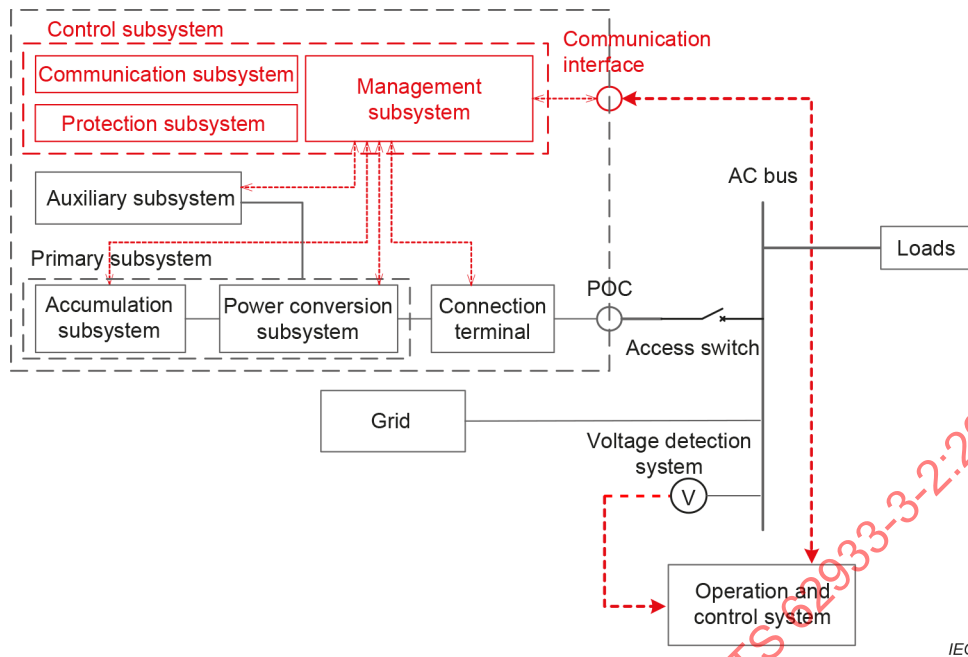
Figure 22 – Example of the system structure of the EES system for grid voltage support
