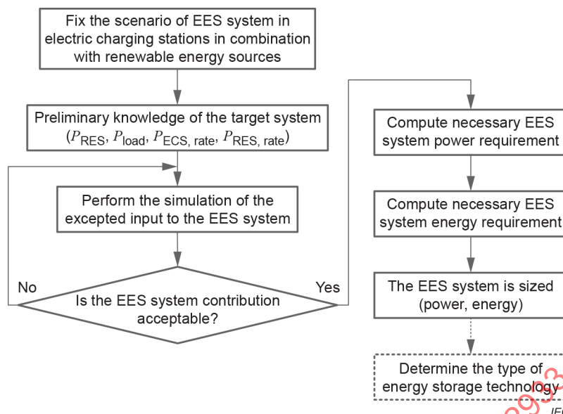
Figure 39 – Example of EES system sizing process of the EES system in electric charging stations in combination with renewable energy sources
