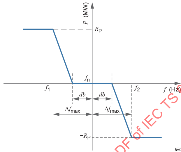
Figure 8 – Example of droop control with frequency dead band
