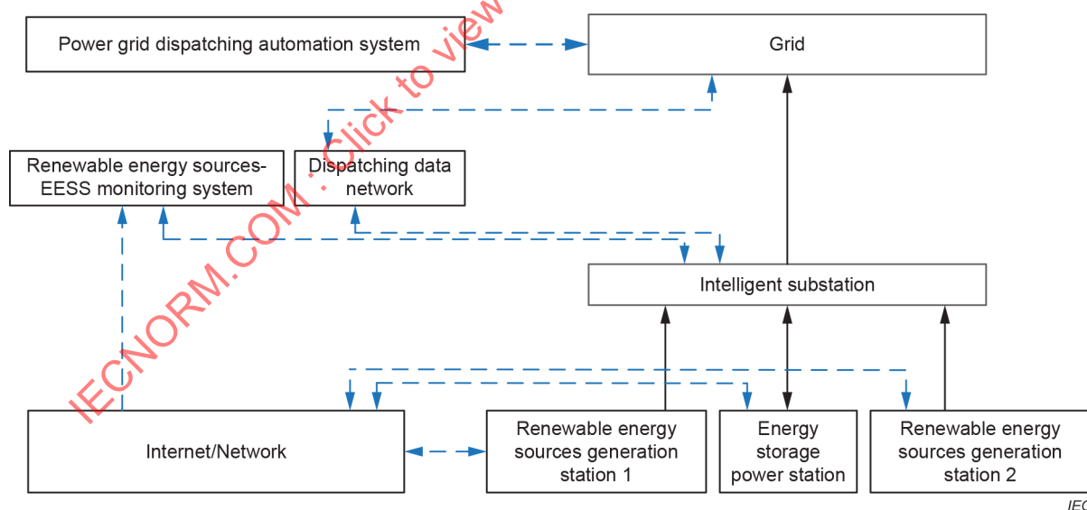
Figure 35 – Example of the EES system for renewable energy sources (power) monitoring system
