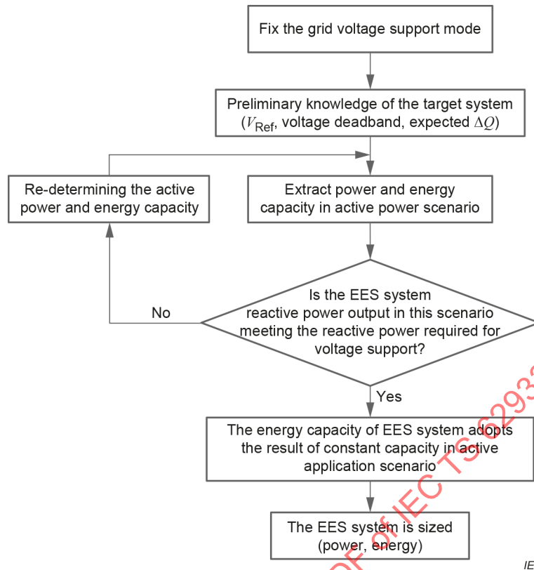
Figure 24 – Example of EES system sizing process for voltage support
