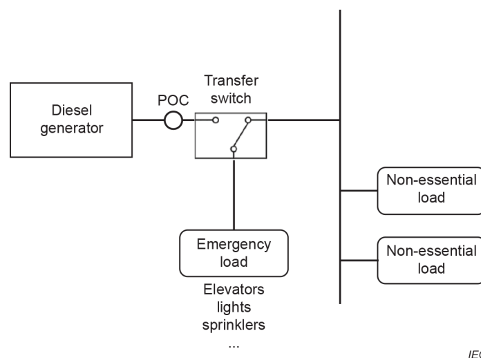
Figure 10 – Example use case for backup power using a diesel generator
