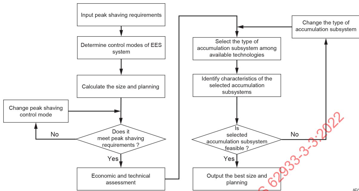
Figure 5 – Process to determine the sizing and planning of the EES system applied in peak shaving and fluctuation reduction of consumption applications
