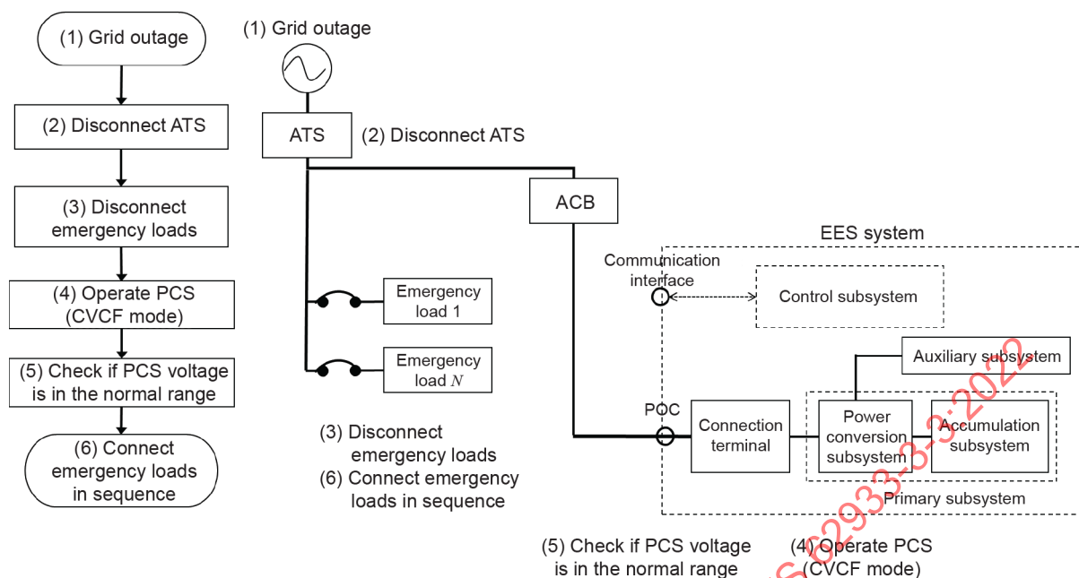
Figure 15 – Example operation flow for backup power support during grid outage
