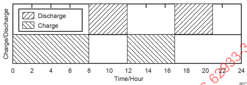
Figure 3 – Two charges and two discharges duty cycle for peak shaving application
