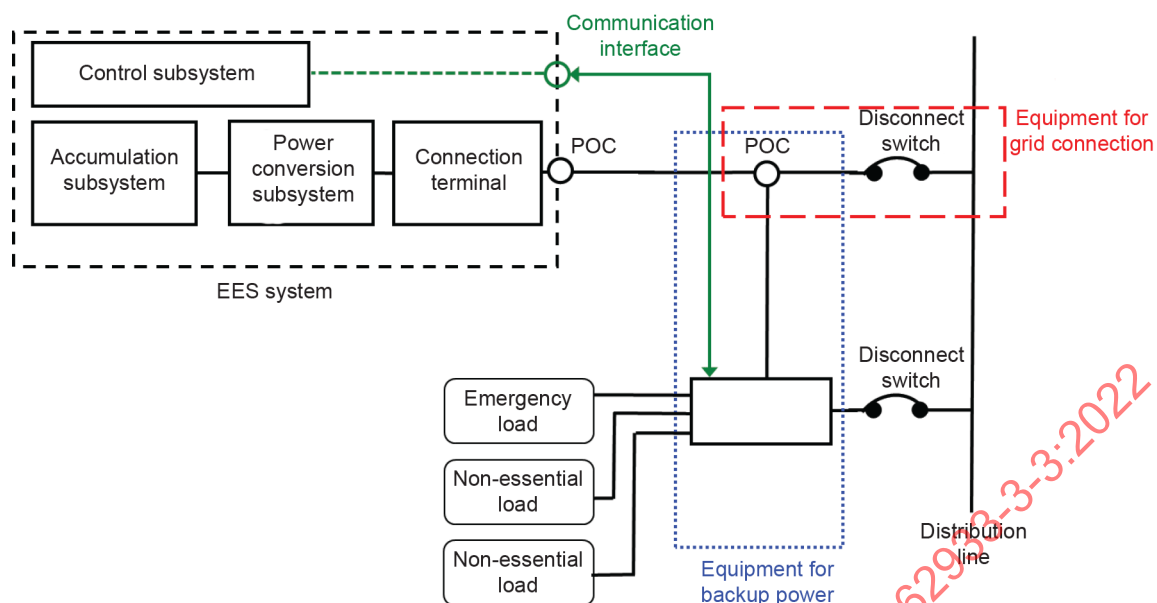
Figure 13 – EES system use case for communication with distribution panel
