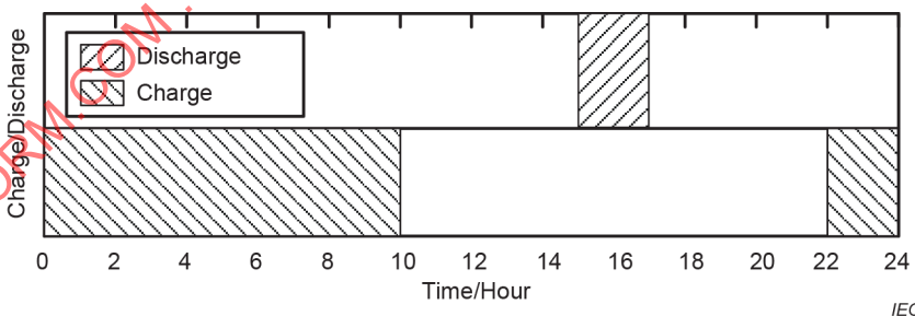
c) Peak shaving duty cycle C, 2 h discharge
