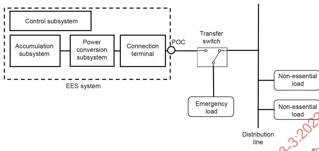
Figure 11 – Simple replacement of diesel generator with EES system for backup power support
