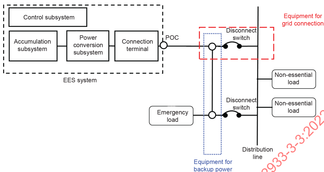
Figure 12 – EES system use case for both backup power and EES's own functions
