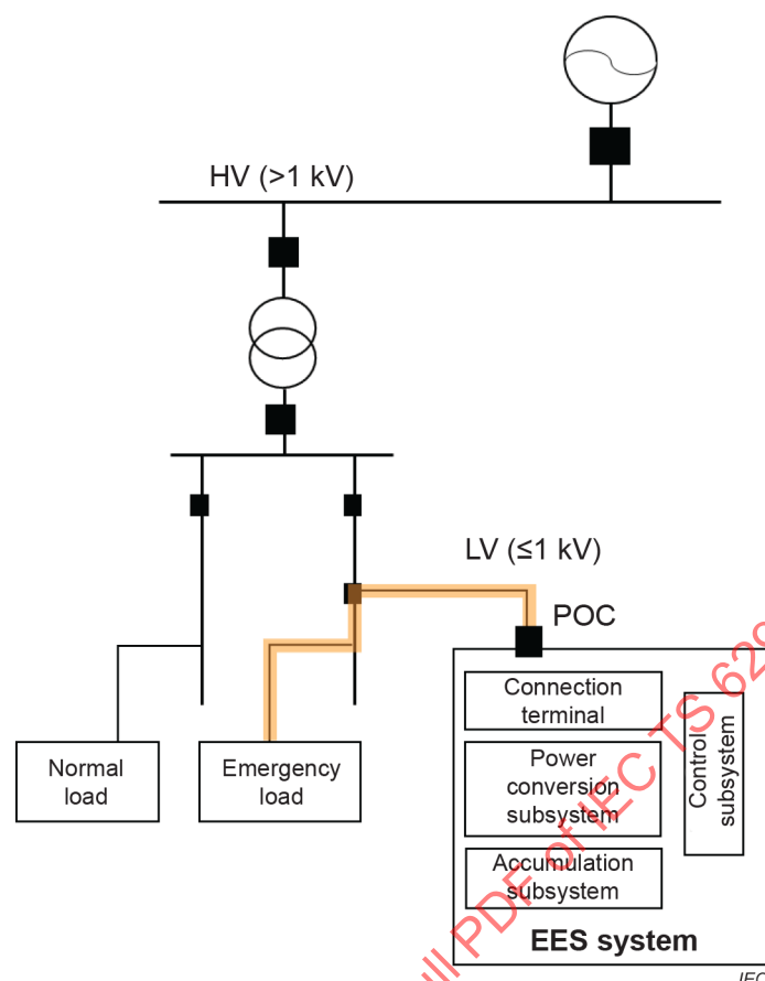
Figure 17 – Example of configuration for low voltage connection
