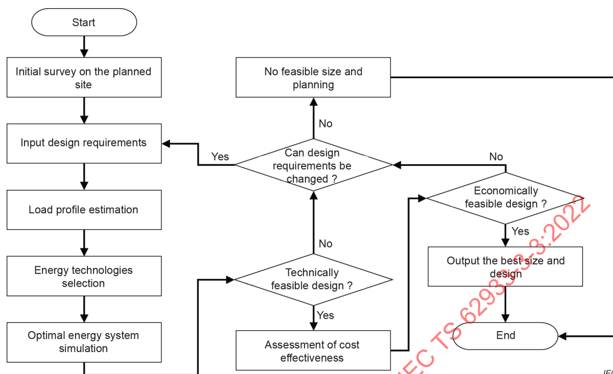
Figure 9 – Example process to determine the sizing and planning of the EES system applied in islanded grid application
