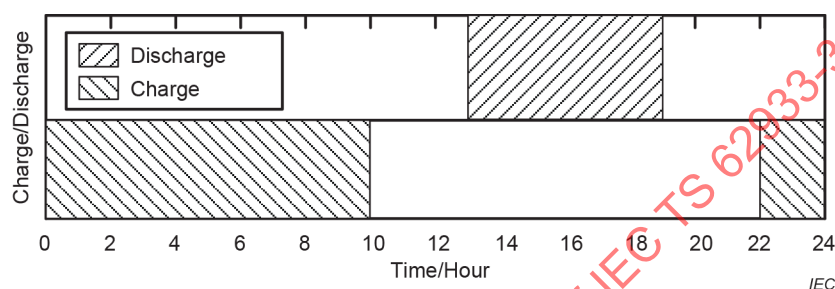
a) Peak shaving duty cycle A, 6 h discharge
