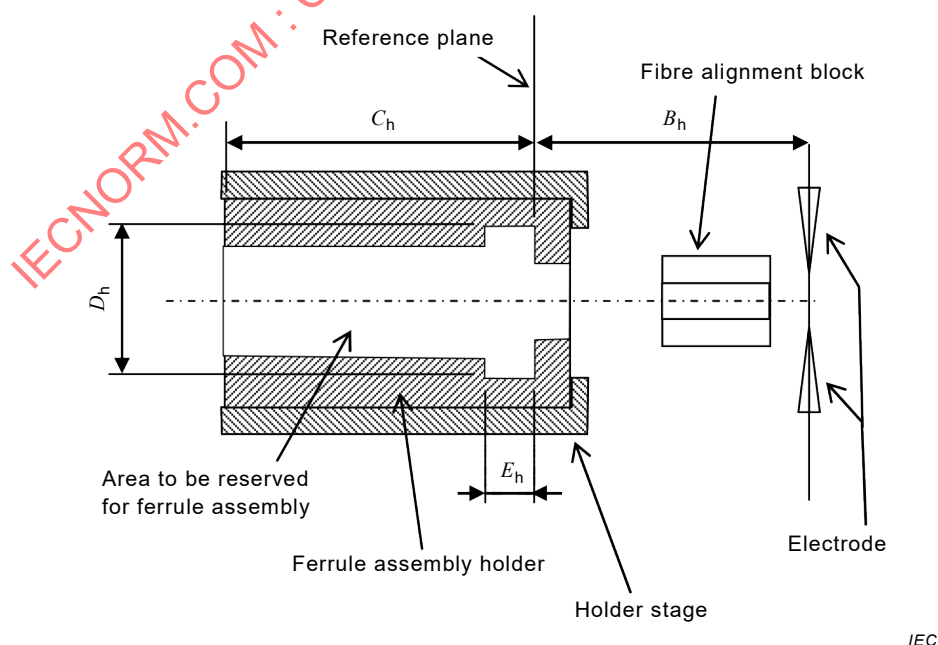
Figure A.1 – An example of a universal holder interface
