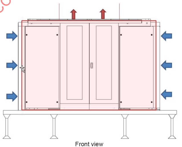
Hot aisle area, boundary and air flow
