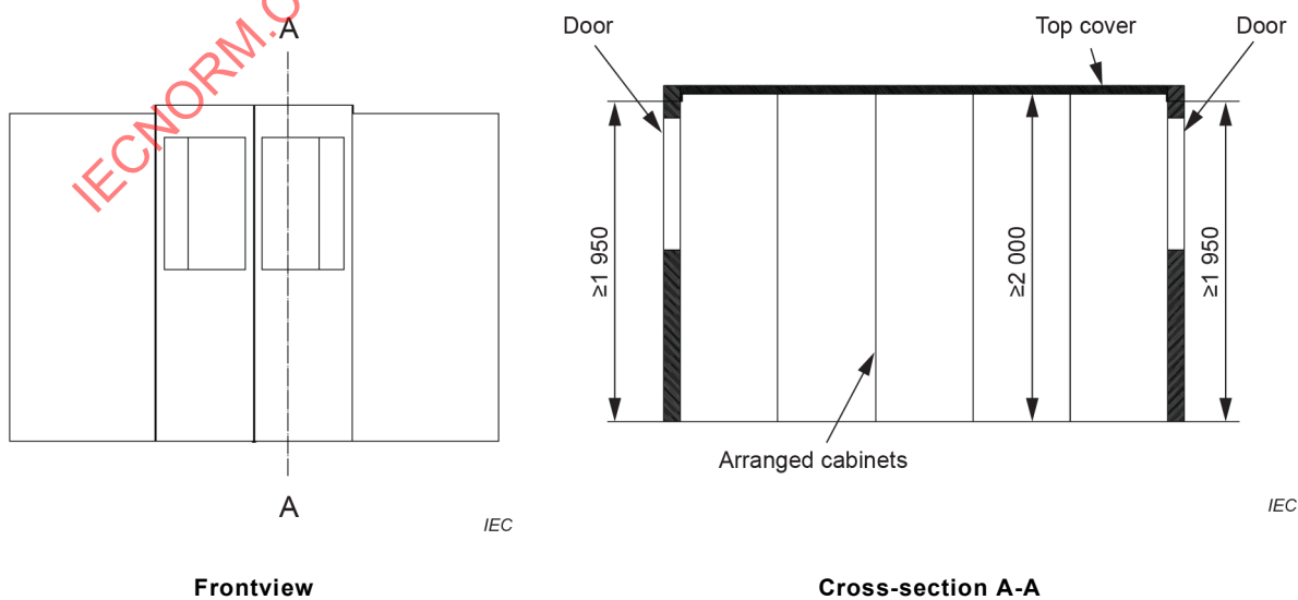
Figure 2 – Minimum height of escape routes in an aisle containment
