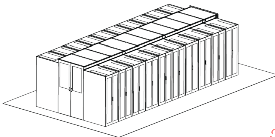
Figure 3 – Typical arrangement of an aisle containment representing a walk-in-equipment solution
