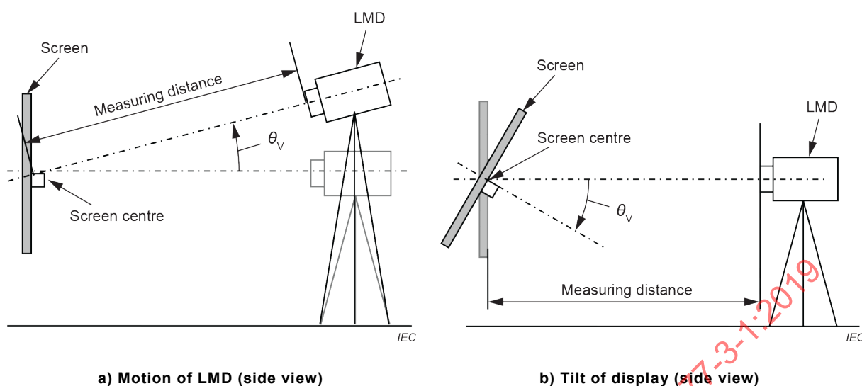
Figure 3 – Measuring layout for vertical viewing direction dependency
