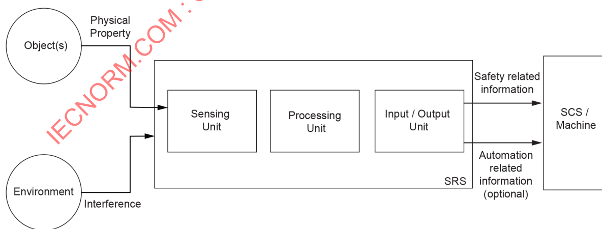
Figure 2 – Example 1 of SRS architecture
