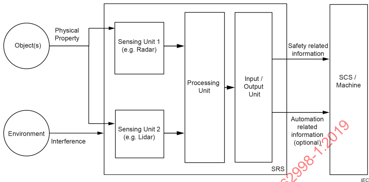
Figure 3 – Example 2 of SRS architecture
