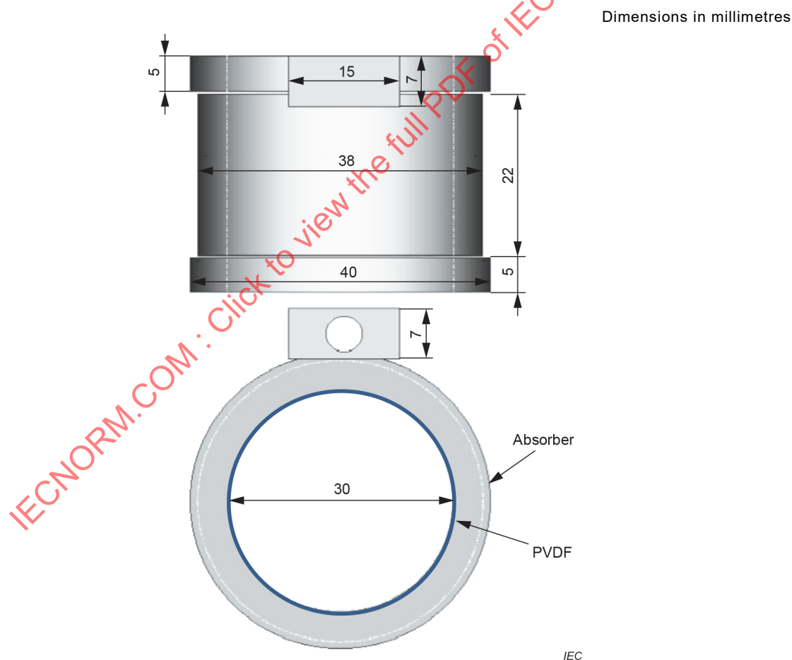
Figure E.1 – Schematic of the cylindrical cavitation hollow cavitation sensor [27], [28]
