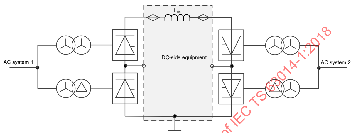
Figure 1 – Scope of DC-side equipment for a back-to-back HVDC converter station with one 12-pulse bridge per end
