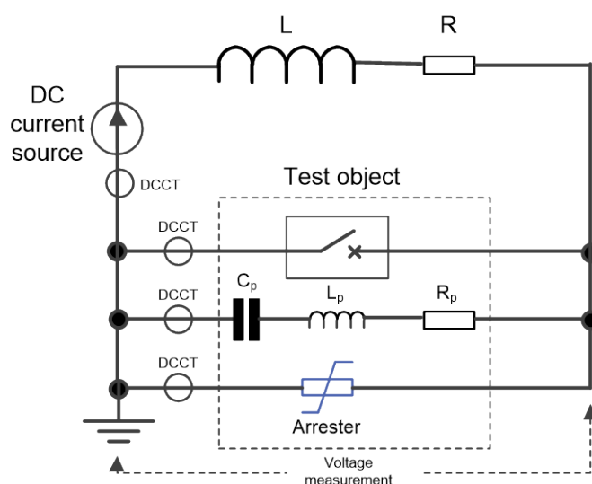
Figure 4 – Test circuit for commutation test
