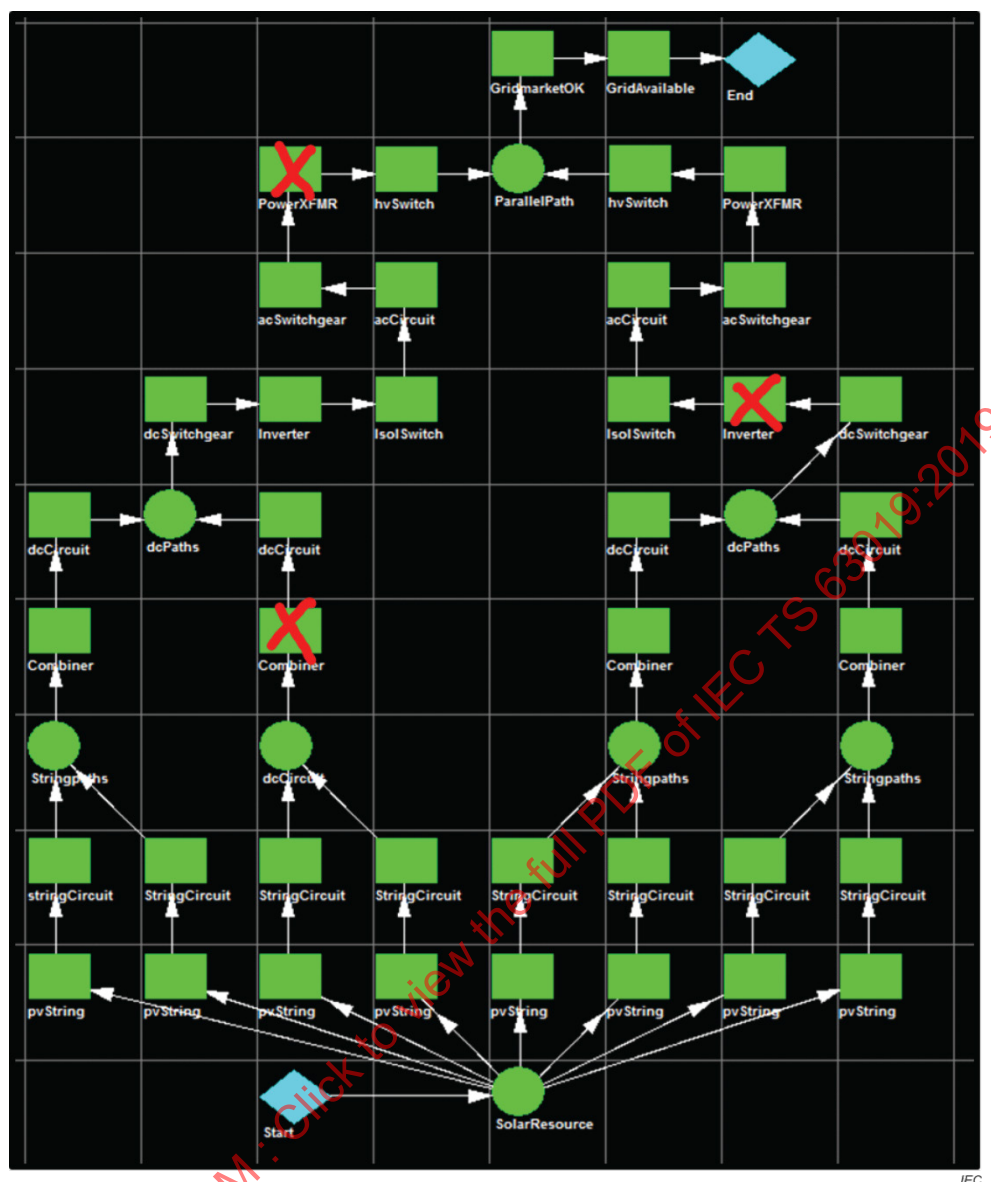
Figure B.1 – RBD of a PVPS
