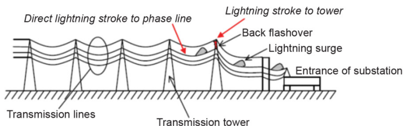
Figure 4 – Overvoltage mechanism caused by back-flashover and direct lightning
