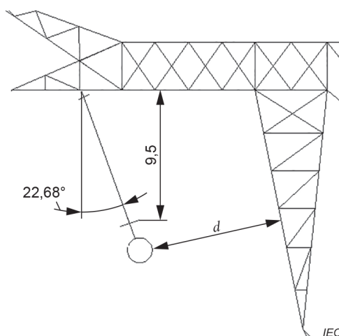
Figure D.12 – The arrangement of switching impulse flashover voltage test for side-phase air clearances of 1 000 kV cup type towers
