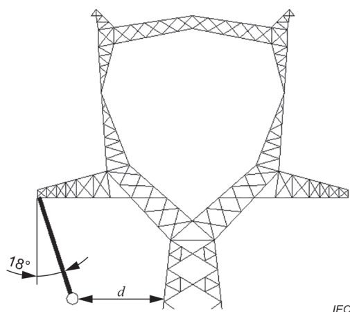
Figure D.9 – The arrangement of switching impulse flashover voltage test for side-phase air clearances of 1 000 kV cat-head type towers
