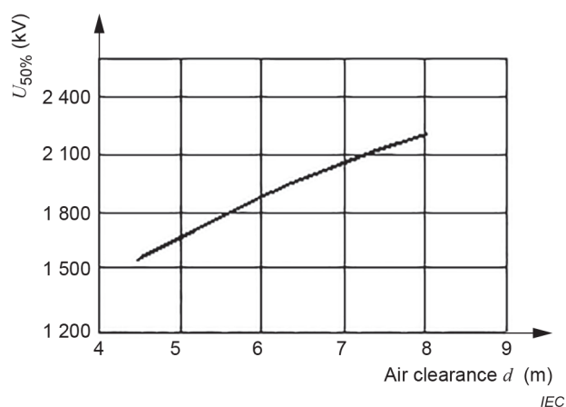
Figure D.13 – The 50 % switching impulse flashover voltage characteristic for air clearances from conductor to tower body of 1 000 kV lines (with a time to peak of 250 \mu s)
