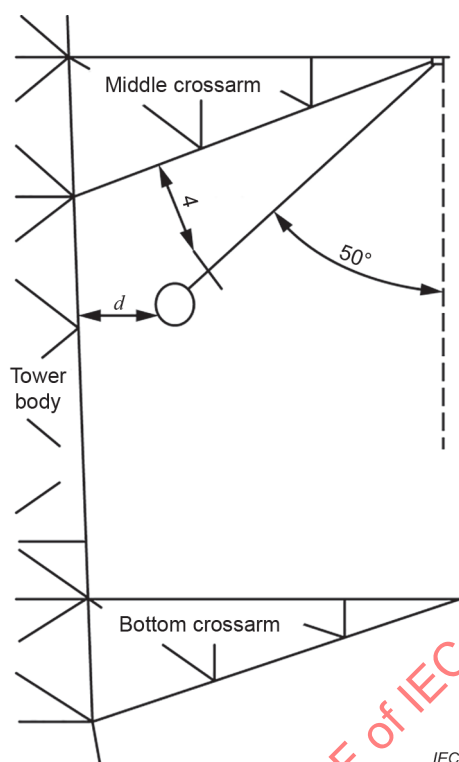
Figure D.5 – The arrangement of power frequency flashover voltage test for air clearances of 1 000 kV double-circuit lines
