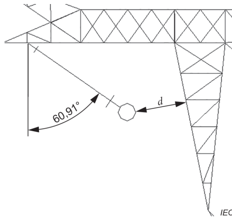
Figure D.3 – The arrangement of power frequency flashover voltage test for side-phase air clearances of 1 000 kV cup type towers.
