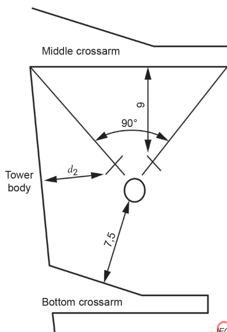
Figure D.19 – The arrangement of switching impulse flashover test for air clearances from middle-phase conductor (with V-type string) to tower body of 1 000 kV double-circuit lines
