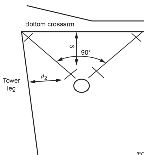
Figure D.25 – The arrangement of switching impulse flashover voltage test for air clearances from bottom-phase conductor (with V-type string) to tower body of 1 000 kV double-circuit lines
