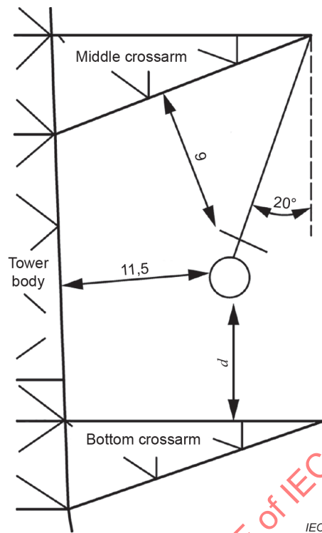
Figure D.15 – The arrangement of switching impulse flashover voltage test at long time to peak for middle-phase air clearances (with I-type string) of 1 000 kV double-circuit lines
