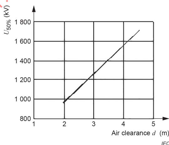
Figure D.2 – The 50 % power frequency flashover voltage characteristic for air clearance from side-phase conductor to tower body for 1 000 kV cat-head type towers
