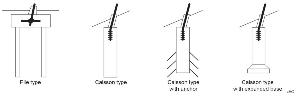
Figure B.12 – Foundation type
