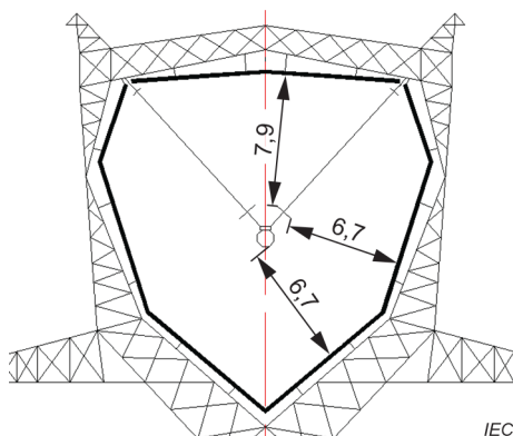
Figure D.11 – The arrangement of switching impulse flashover voltage test for middle-phase air clearances of 1 000 kV cat-head type towers
