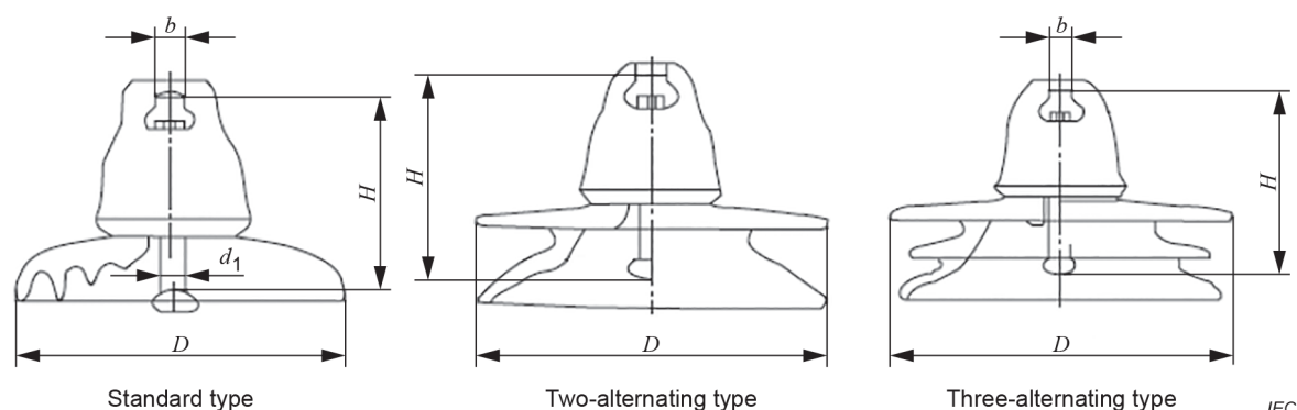
Figure B.2 – 1 200 kV insulator profile
