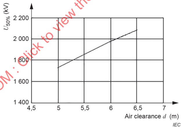
Figure D.20 – The 50 % switching impulse (1 000 \mu s) flashover voltage characteristic for air clearances from conductor to tower body of 1 000 kV double-circuit lines
