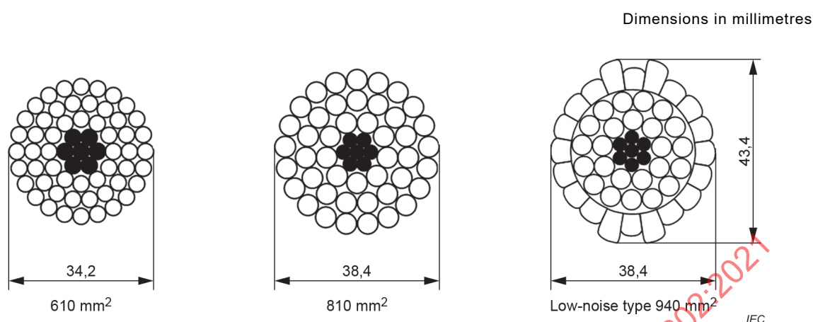
Figure B.10 – Shape of conductor
