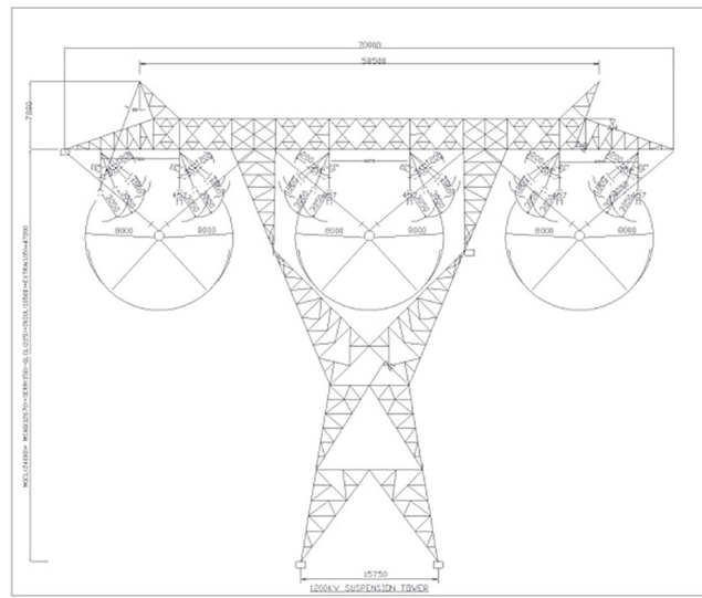
Figure B.6 – 1 200 kV upgradable line –Suspension tower
