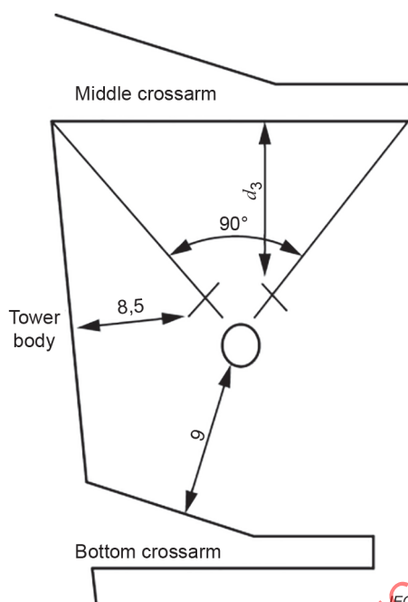
Figure D.21 – The arrangement of switching impulse flashover voltage test for air clearances from middle-phase conductor (with V-type string) to middle crossarm of 1 000 kV double-circuit lines
