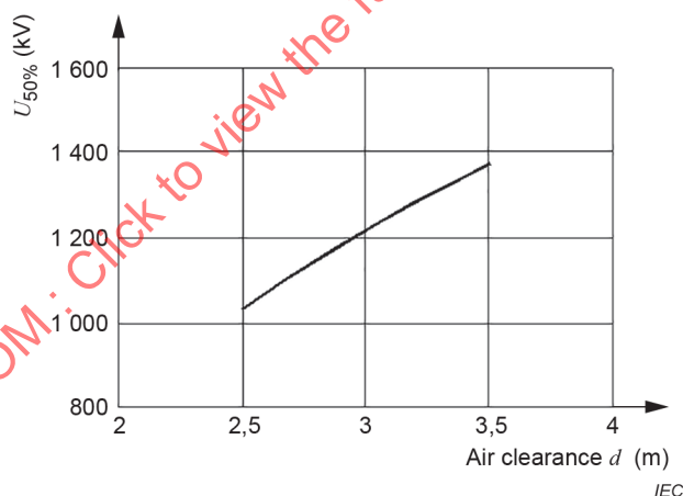
Figure D.8 – The power frequency flashover voltage characteristic of air clearance from bottom-phase conductor (with I-type string) to tower body of 1 000 kV double-circuit lines
