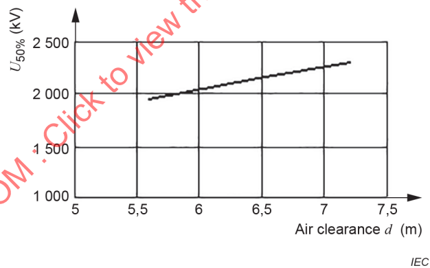
Figure D.16 – The 50 % switching impulse (1 000 \mu s) flashover voltage characteristic for air clearances from conductor to bottom crossarm of 1 000 kV double-circuit lines (a distance of 9,0 m between conductor and middle crossarm)
