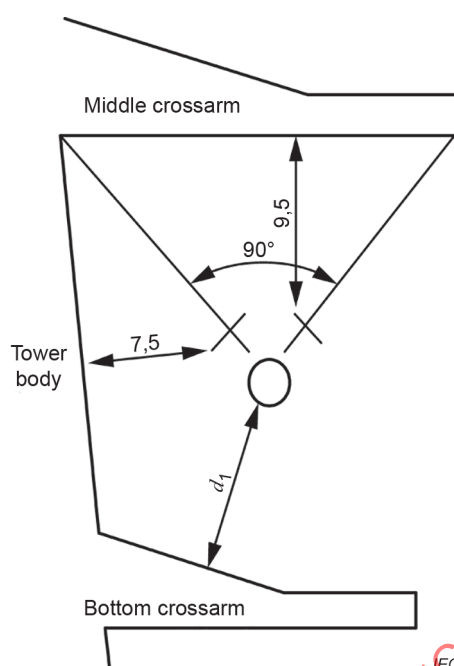
Figure D.17 – The arrangement of switching impulse flashover voltage test for air clearances from middle-phase conductor (with V-type string) to bottom crossarm of 1 000 kV double-circuit lines
