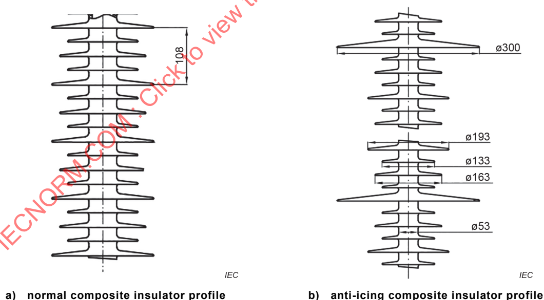
Figure B.1 – Composite insulator profiles
