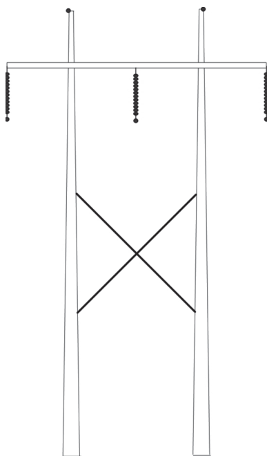
Figure 5 – Typical single circuit H-type tower
