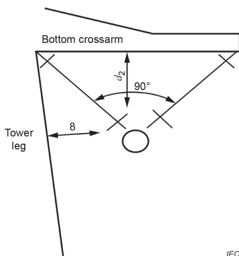
Figure D.23 – The arrangement of switching impulse flashover voltage test for air clearances from bottom-phase conductor (with V-type string) to crossarm of 1 000 kV double-circuit lines
