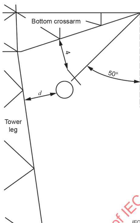
Figure D.7 – The arrangement of the power frequency flashover voltage test for air clearances of bottom-phase with I-type string of 1 000 kV double-circuit lines
