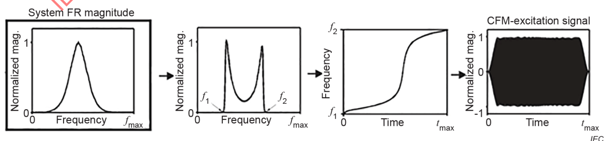
Figure 3 – Development and signal processing for a compensated frequency modulated signal
