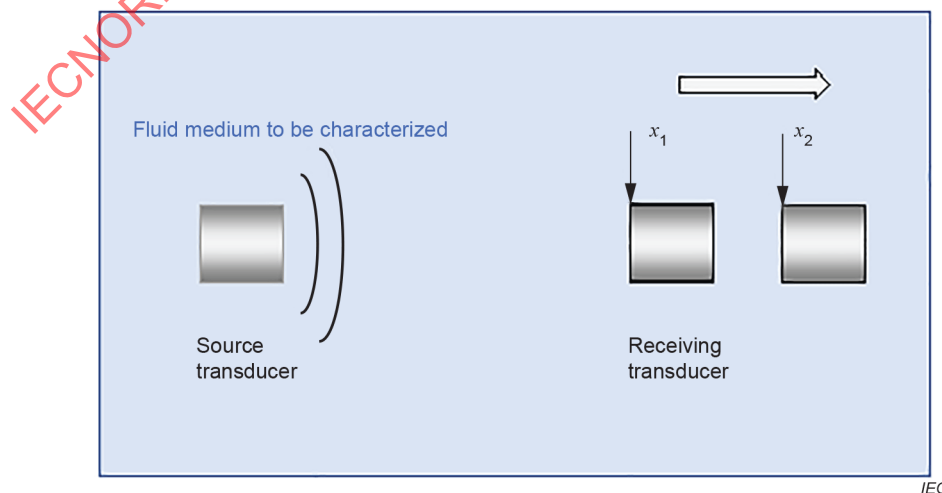
Figure 6 – Source and receiving transducers immersed in a fluid medium to be characterized
