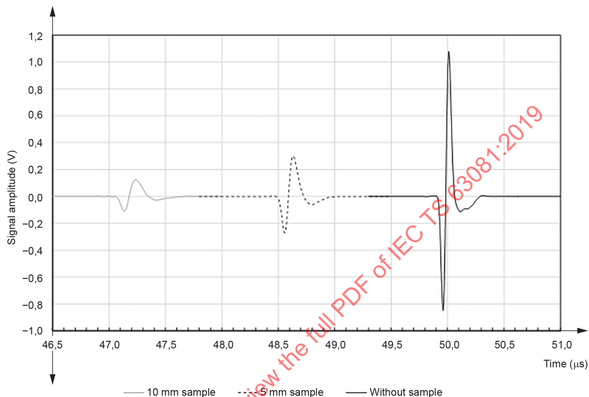
Figure 4 – Pulse dispersion in absorbing media
