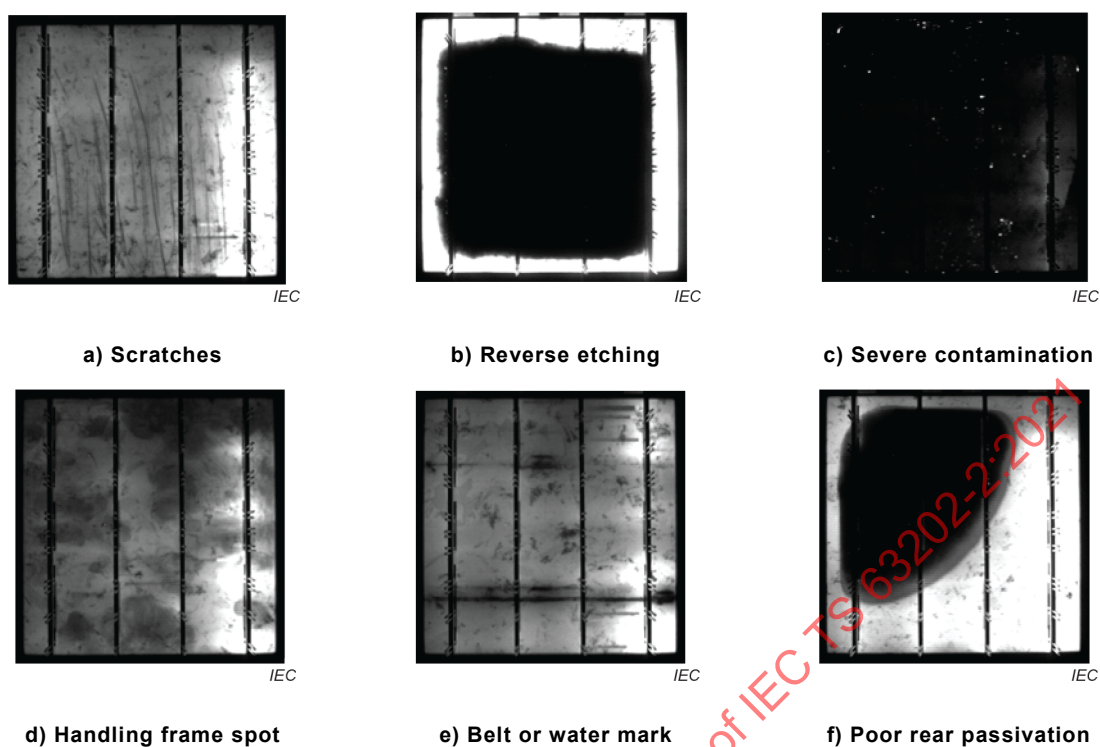
Figure 7 – EL images of PV multi-crystalline silicon solar cells
