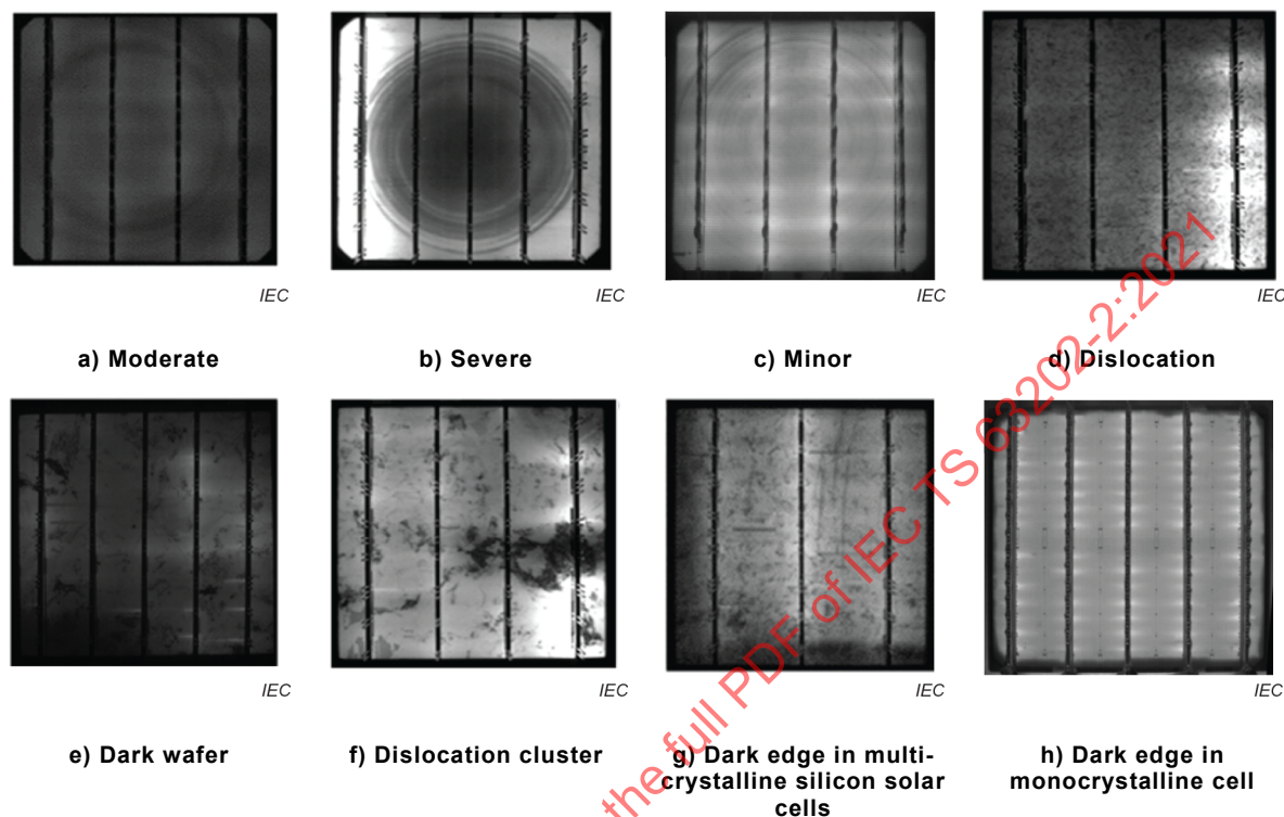
Figure 4 – EL images of PV cell with different grades of concentric circles in mono-crystalline silicon
