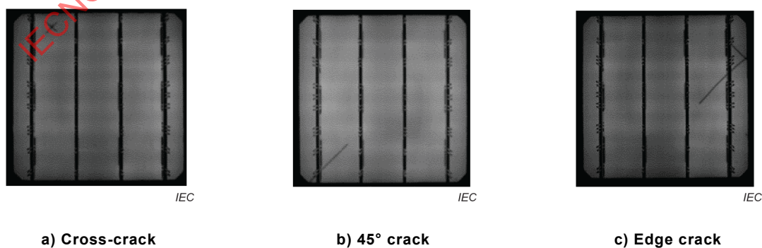
Figure 8 – EL images of PV cell
