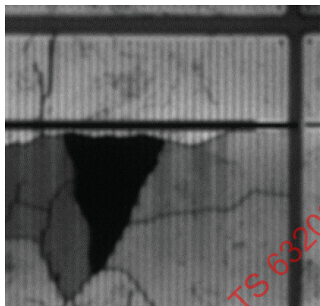
Figure 2 – Image of multi-crystalline silicon solar cell with SNR_{50} value of 45
