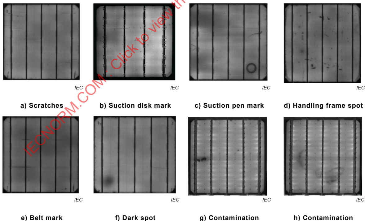
Figure 6 – EL images of PV mono-crystalline silicon solar cells
