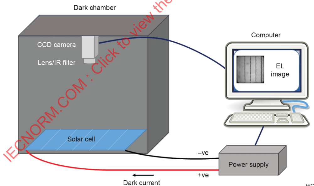
Figure 1 – Typical setup of an electroluminescence imaging system
