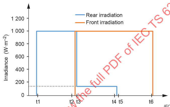
Figure 1 – Schematic procedure of double-side simultaneous irradiation method with integrated flash conditions
