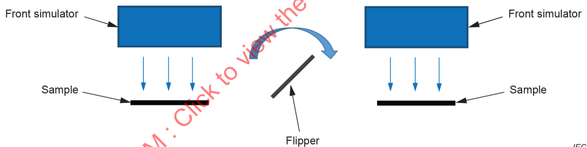
Figure 7 – Schematic configuration with two consecutive solar simulators
