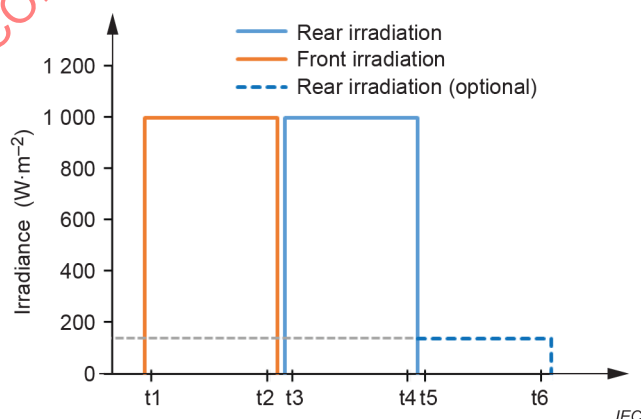
Figure 4 – Schematic procedure of sequential irradiation method with integrated flash conditions
