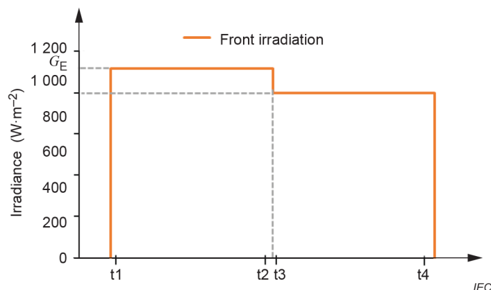
Figure 3 – Schematic procedure of equivalent irradiation method with integrated flash conditions
