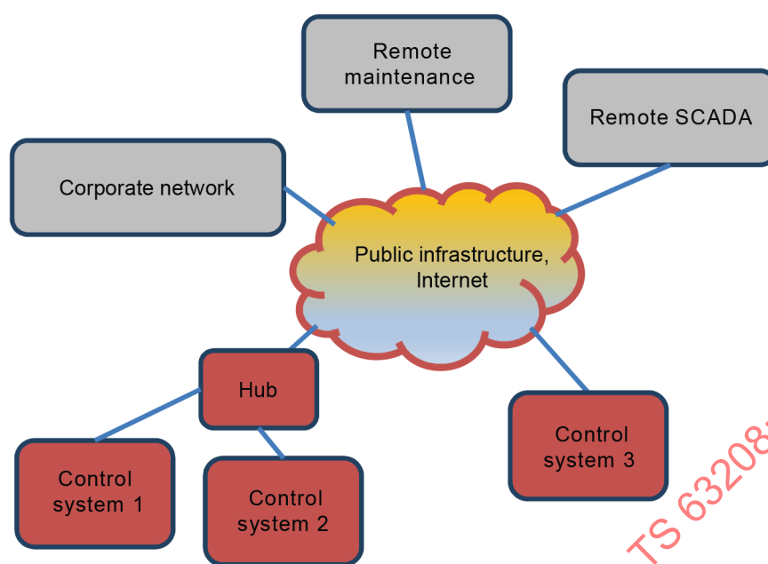
Figure 5 – Control system connectivity level C5
