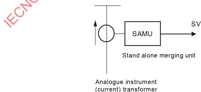
Figure 3 – Analogue transformer connected to a SAMU
