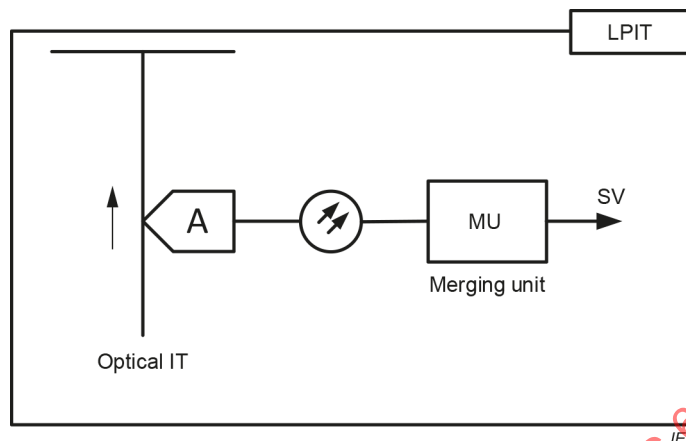
Figure 1 – Example of an optical instrument transformer with digital output (LPIT)
