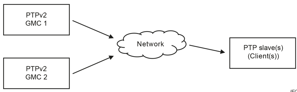
Figure 8 – Communication scheme of PTP IEC/IEEE 61850-9-3
