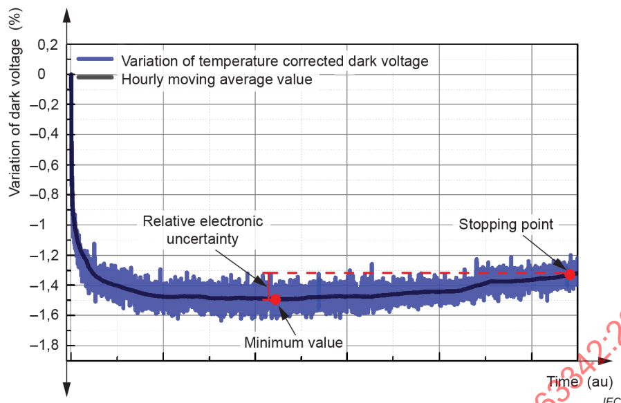
Figure 2 – Dark voltage diagram showing the evolution of the temperature corrected dark voltage over time in arbitrary units during LETID degradation used to identify the time of maximum degradation and the time to stop the LETID degradation sequence
