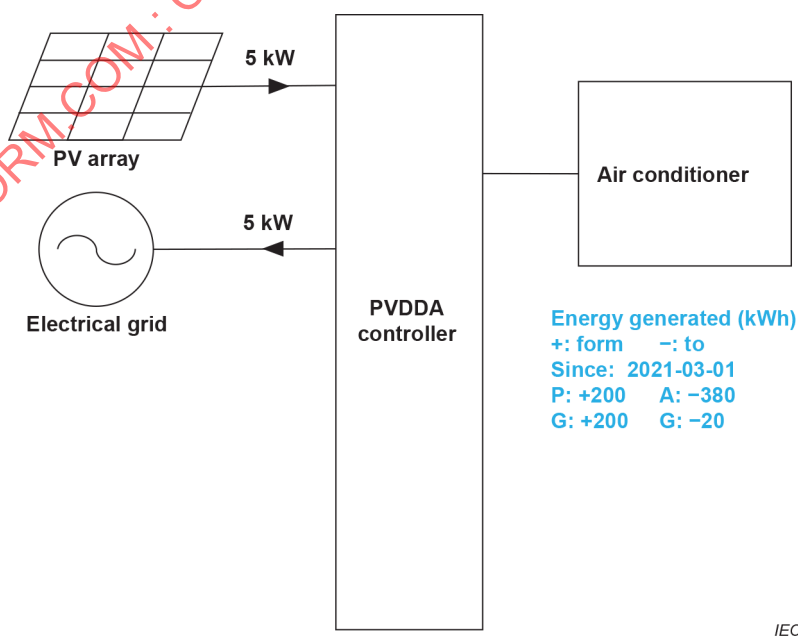
Figure 3 – Display of operation mode PAG//P→G
