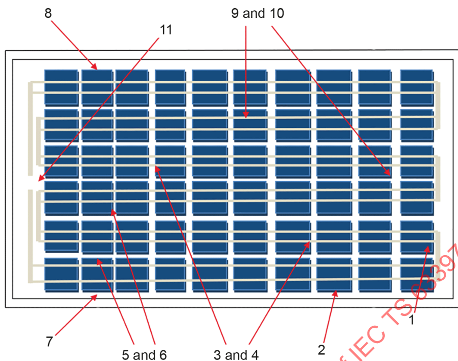
a) Impact locations for wafer/cell based technologies
