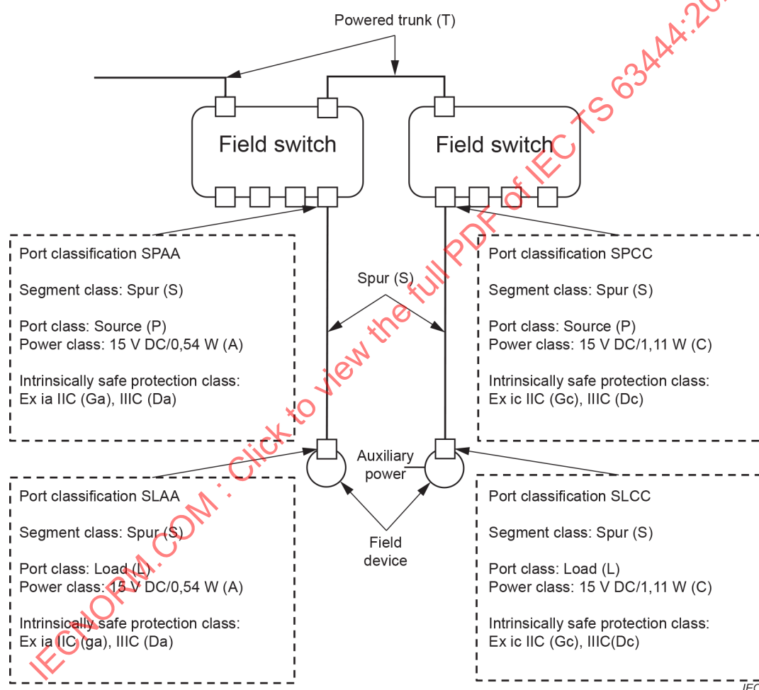
Figure 7 – Example of intrinsically safe protection class matching to port class and power class
