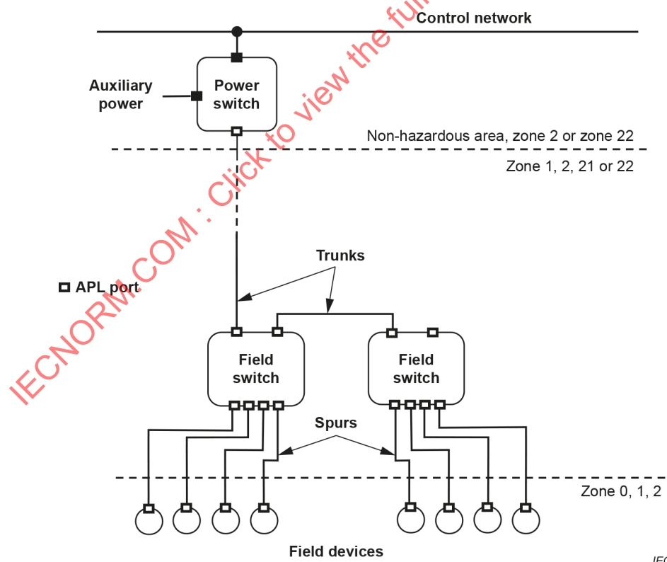
Figure 1 – APL topology example
