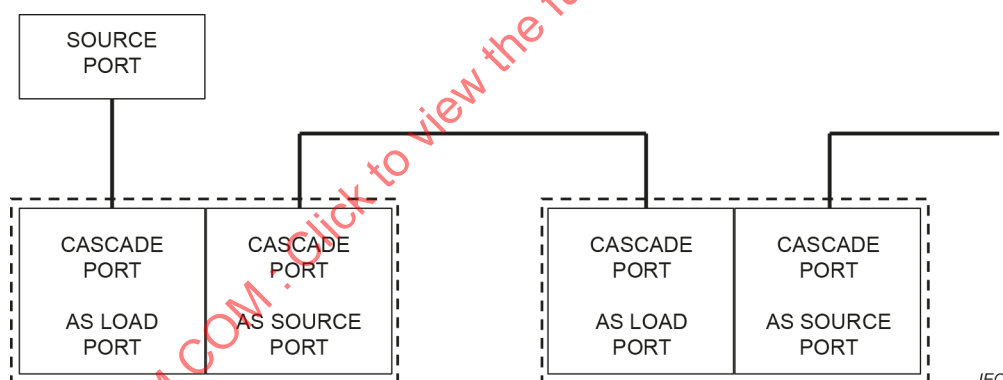
Figure 4 – Powered trunk segments with cascade ports
