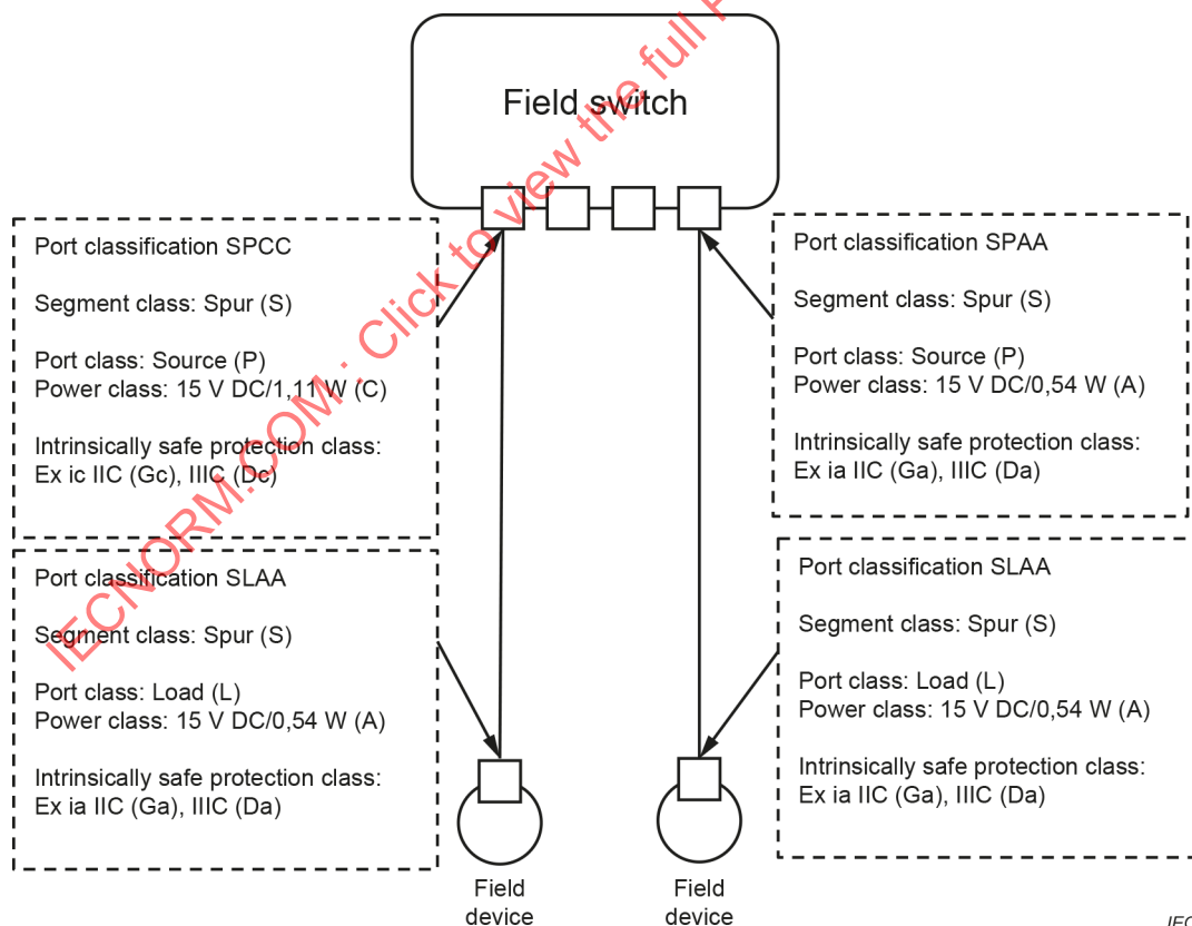
Figure 5 – Example of port class matching between source and load
