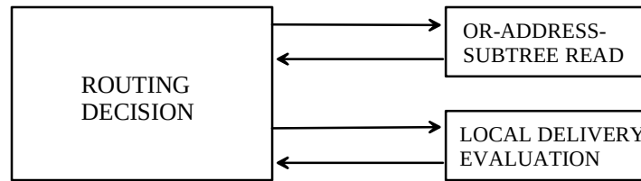
Figure 3 - Organization of procedures within the Routing-decision procedure
