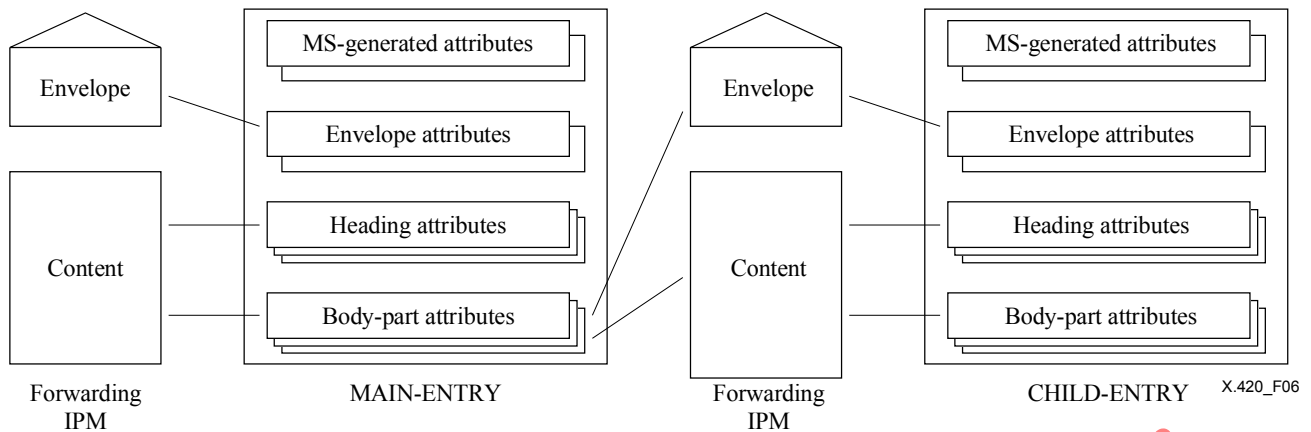
Figure 6 – Mapping a Forwarding message to an IPMS-MS entry
