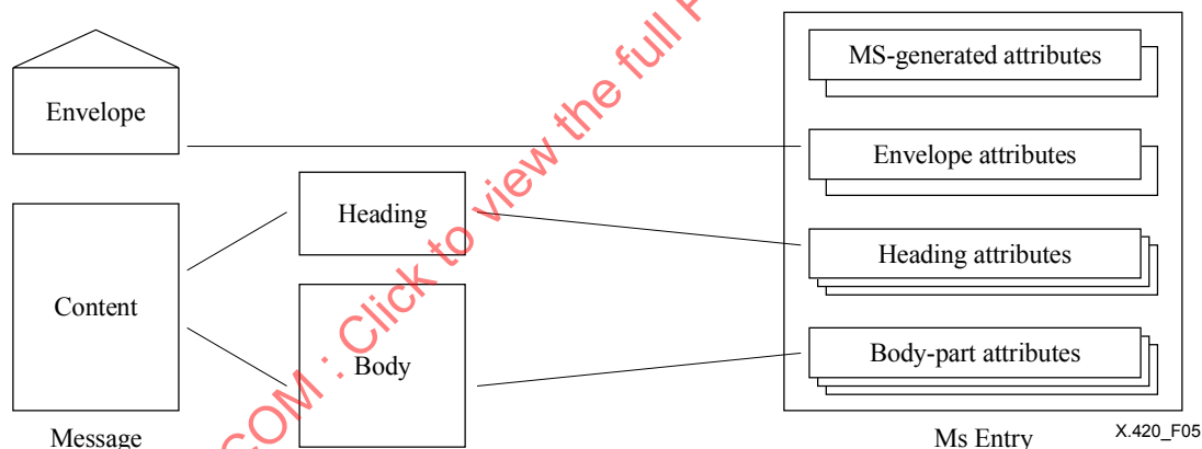
Figure 5 – Mapping an IPM to an Ms entry
