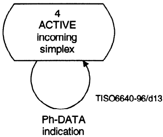
Figure 12 – State transition diagram for simplex mode, incoming, data transfer phase only
