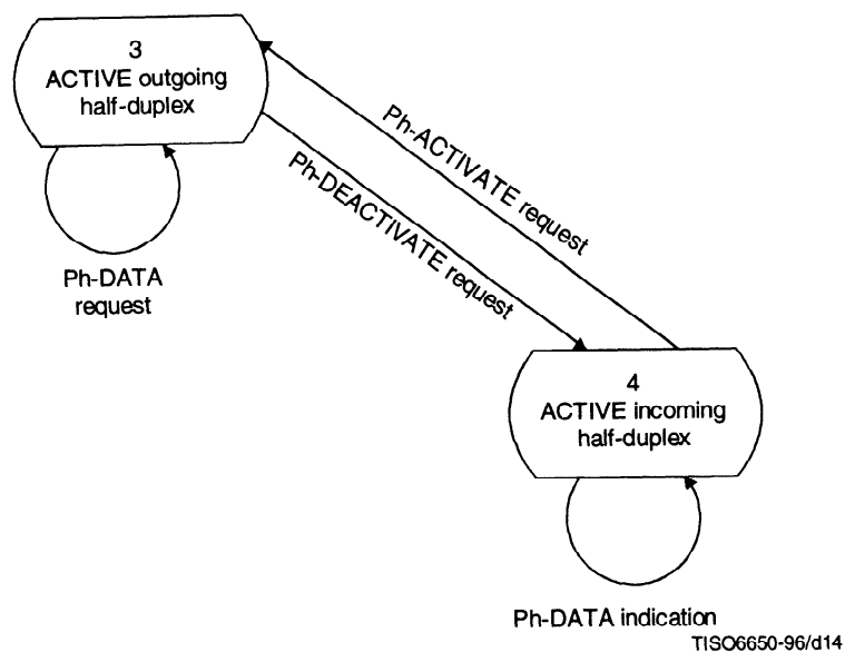
Figure 13 – State transition diagram for half-duplex mode without inactive state
