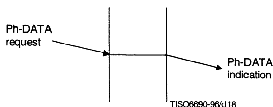
Figure 17 – Sequence of primitives in data transfer
