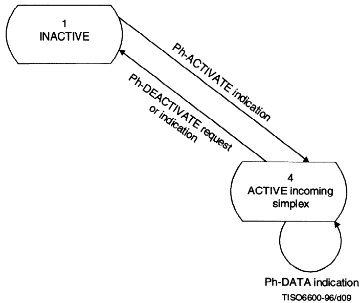
Figure 8 – State transition diagram for simplex mode, incoming
