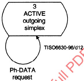
Figure 11 – State transition diagram for simplex mode, outgoing, data transfer phase only
