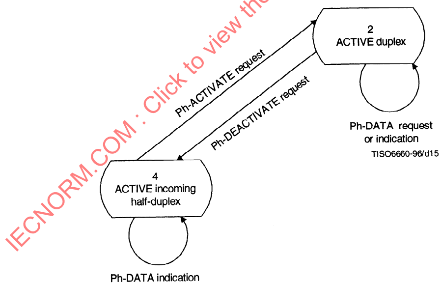
Figure 14 – State transition diagram for half-duplex/duplex mode shift
