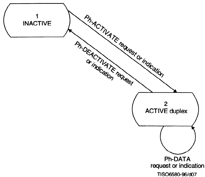
Figure 6 – State transition diagram for duplex mode with Activation/Deactivation
