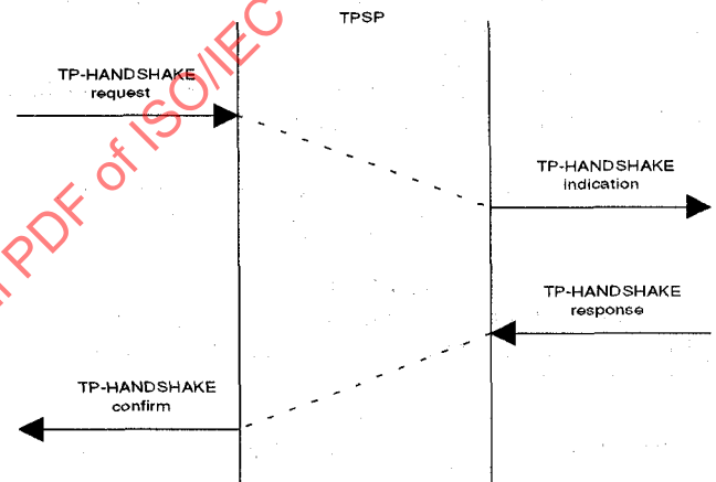
Figure 11 - TP-HANDSHAKE sequence of primitives
